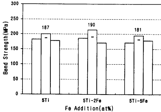
Fig 5. Four-point bend strength of the SiC/SiC joints brazed by the Ag-5at%Ti and -5at%Fe alloys. (values in the graph : mean bend strength)
