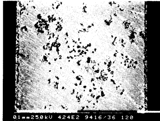
(a) Ag-5at%Ti-2at%Fe
