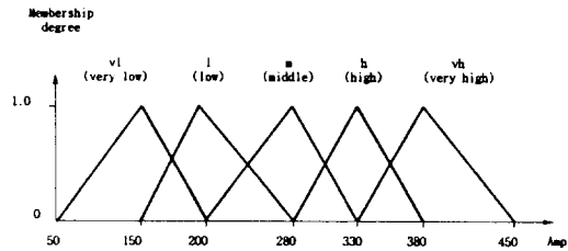
Fig. 5 Evaluation of welding current using fuzzy set
