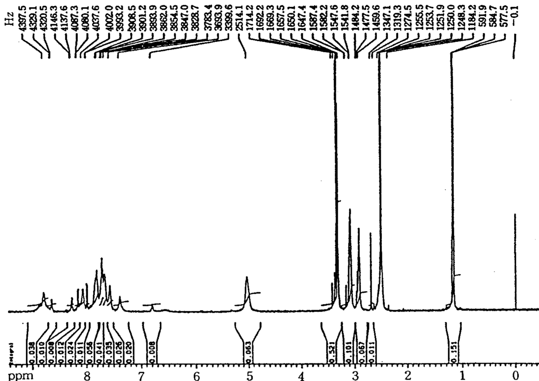
Fig. 4. 1 H-NMR spectrum of 9-phenyl-3,3'-bis(3-sulfopropyl)-4,5,4',5'-naphthothiazolo carbocyanine triethyl ammonium salt.
