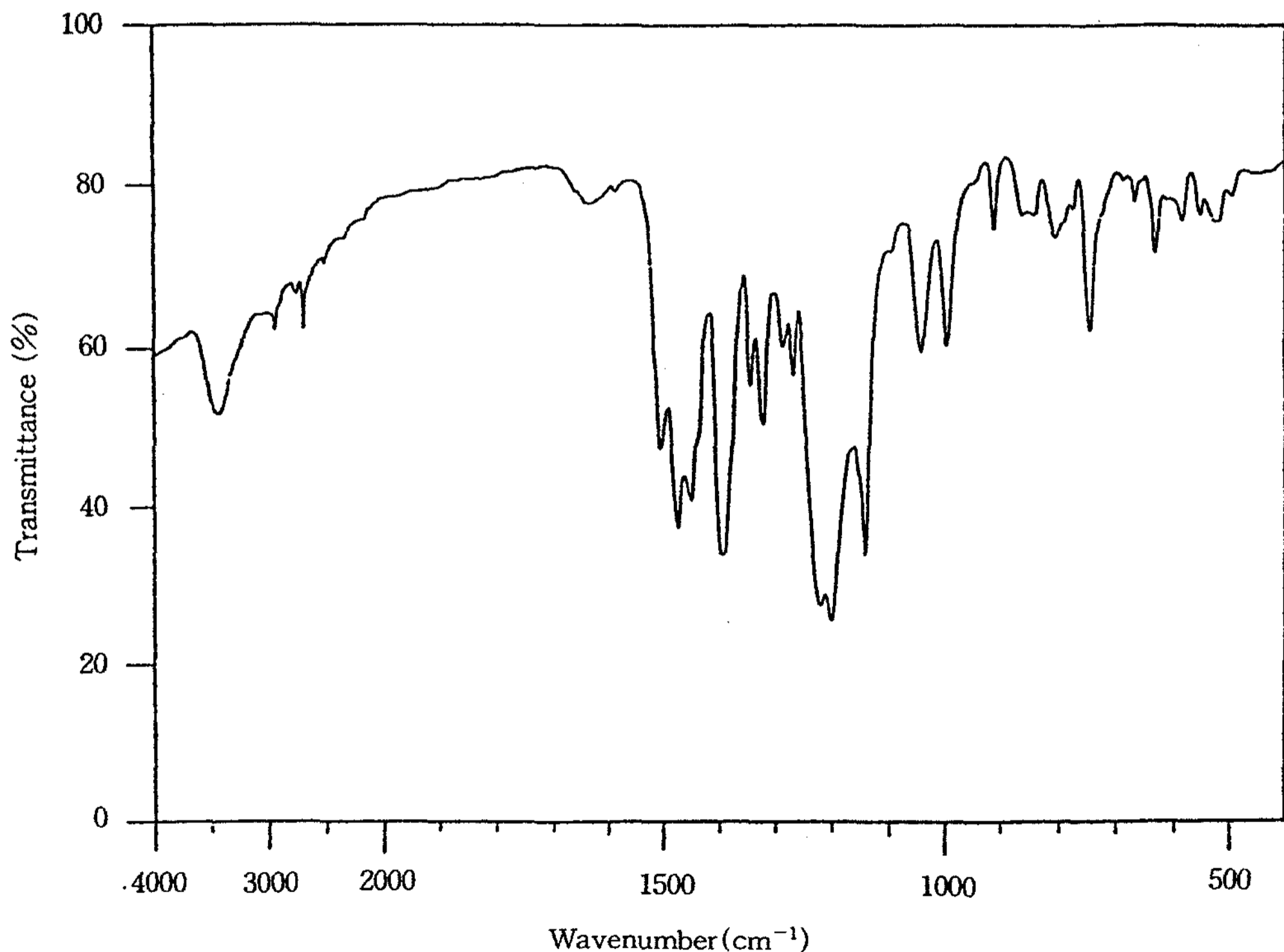
Fig. 1. IR spectrum of 9-phenyl-3,3'-bis(3-sulfopropyl)-4,5,4',5'-naphthothiazolo carbocyanine triethyl ammonium salt.
