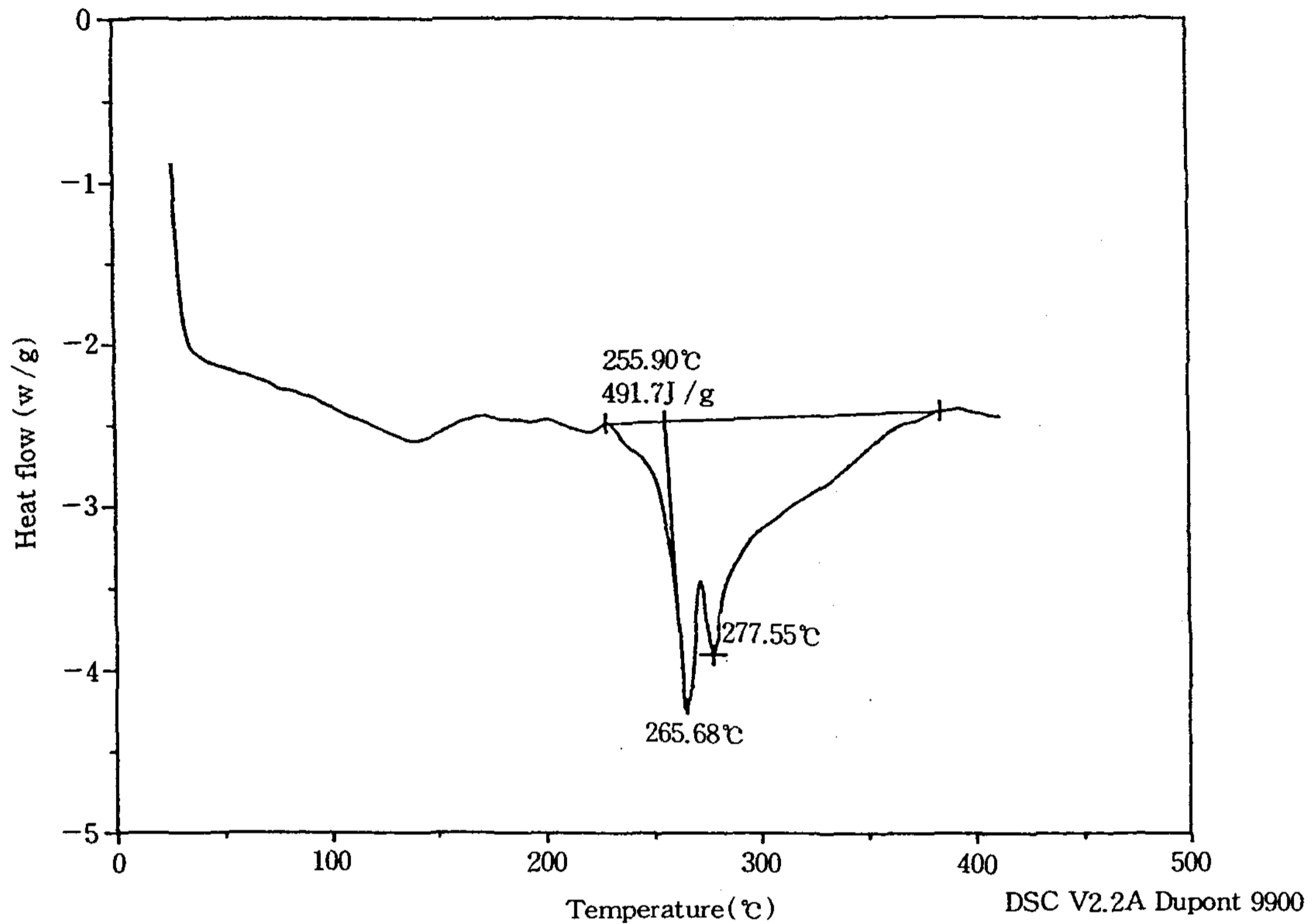
Fig. 6. DSC thermogram of 9-phenyl-3,3'-bis(3-sulfopropyl)-4,5,4',5'-naphthothiazolo carbocyanine triethyl ammonium salt.
