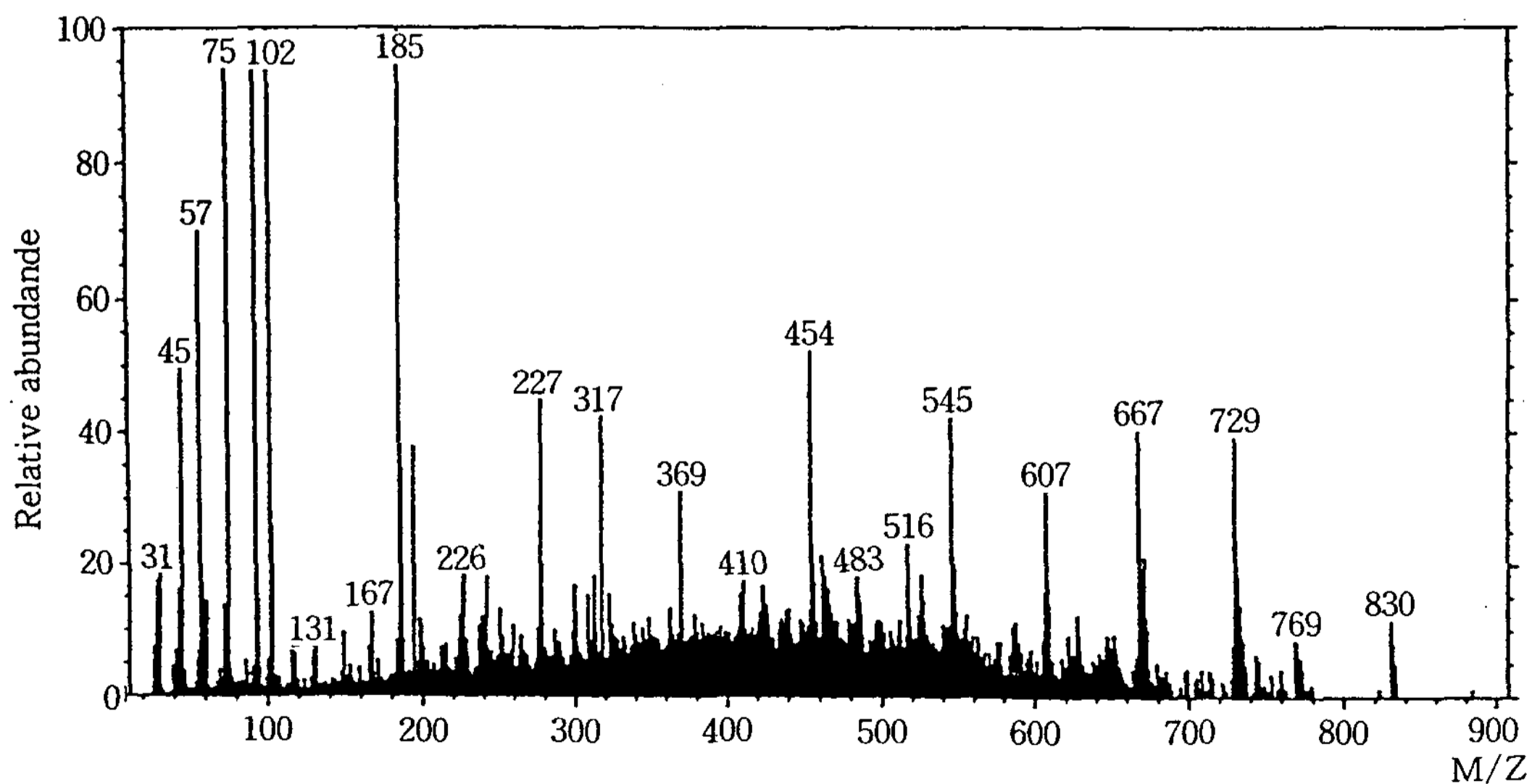
Fig. 3. Positive FAB spectrum of 9-phenyl-3,3'-bis(3-sulfopropyl)-4,5,4',5'-naphthothiazolo carbocyanine triethyl ammonium salt.
