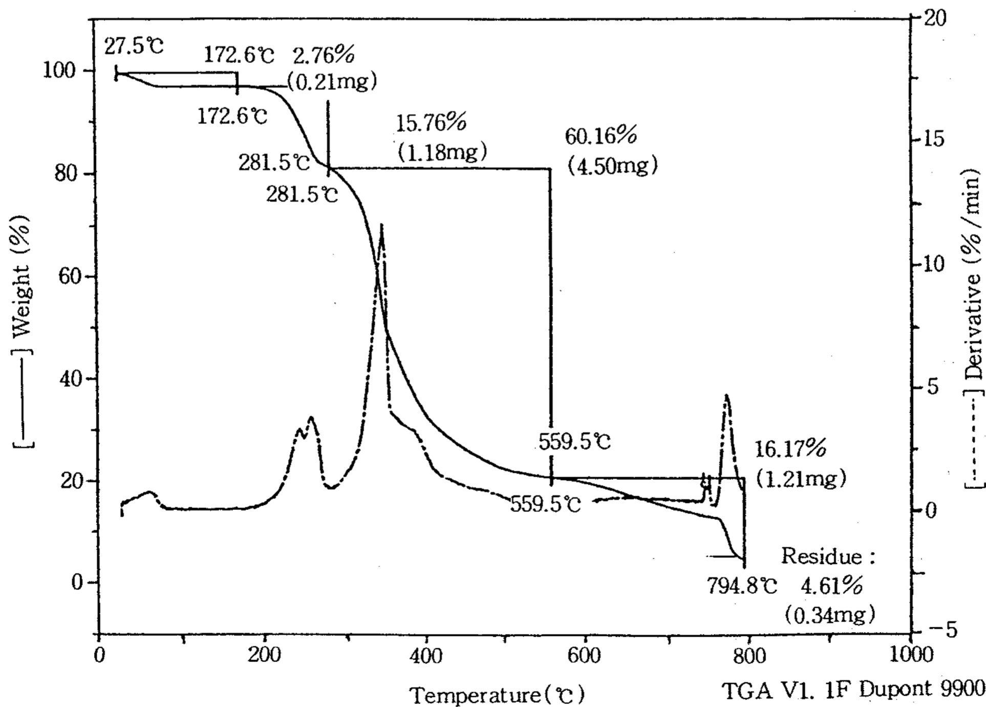
Fig. 5. TGA thermogram of 9-phenyl-3,3'-bis(3-sulfopropyl)-4,5,4',5'-naphthothiazolo carbocyanine triethyl ammonium salt.
