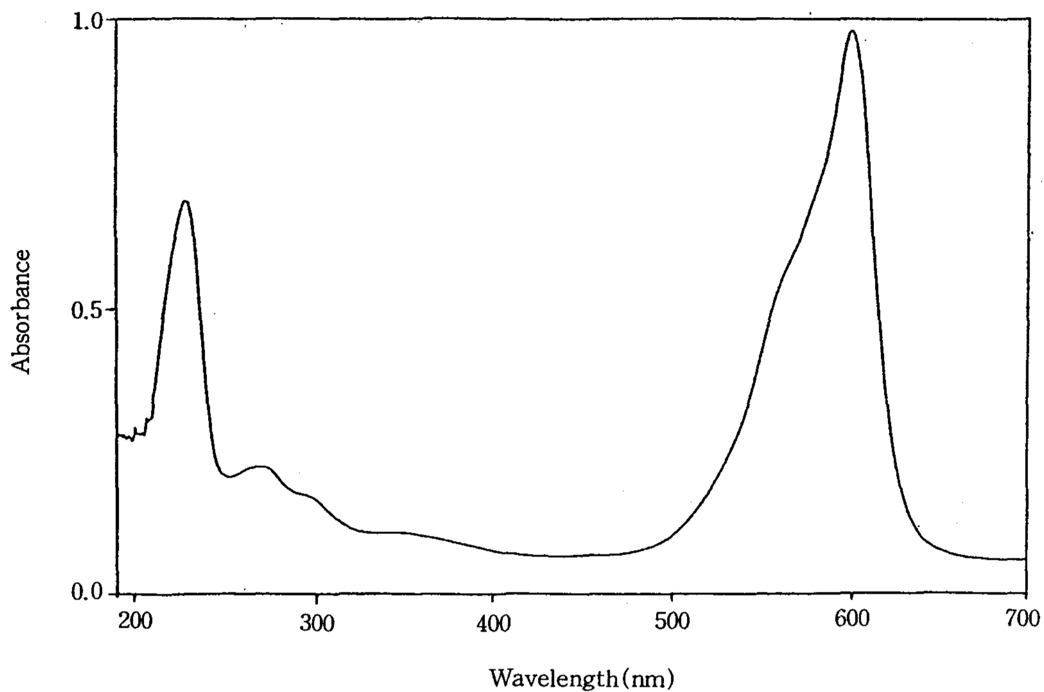
Fig. 2. UV spectrum of 9-phenyl-3,3'-bis(3-sulfopropyl)-4,5,4',5'-naphthothiazolo carbocyanine triethyl ammonium salt.
