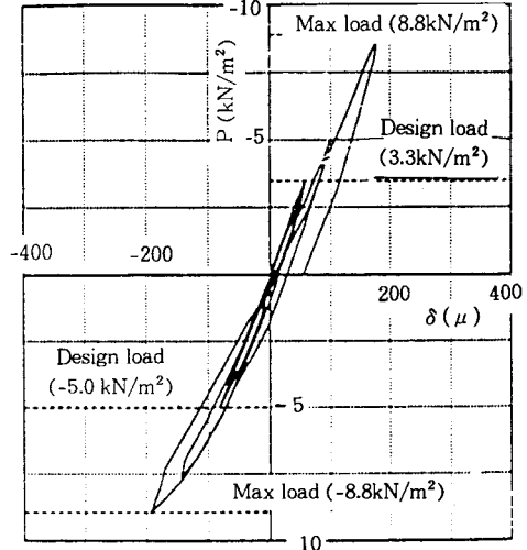
(Wind load vs. strain)
