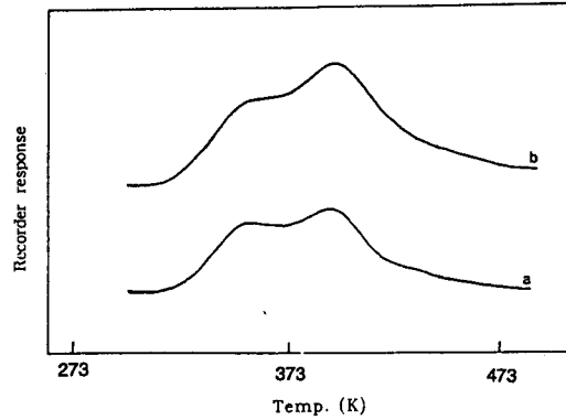
Fig. 5. The TPD thermograms of methylamine adsorbed in dealuminated SAPO-11. a: SAPO-11, b: 24h-dealuminated SAPO-11.
