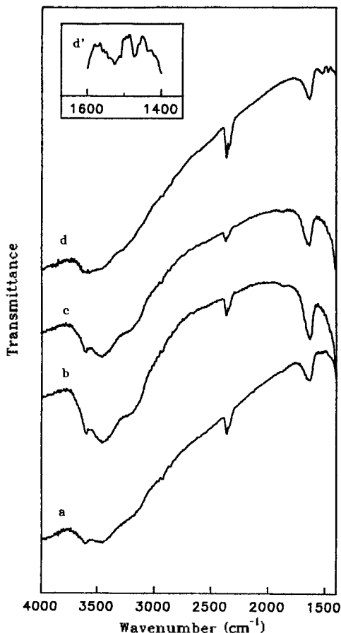
Fig. 3. The IR spectra of dealuminated SAPO-11. a: SAPO-11, b: 12h-dealuminated SAPO-11, c: 24h-dealuminated SAPO-11, d: 24h-dealuminated SAPO-11 after methylamine adsorption.
