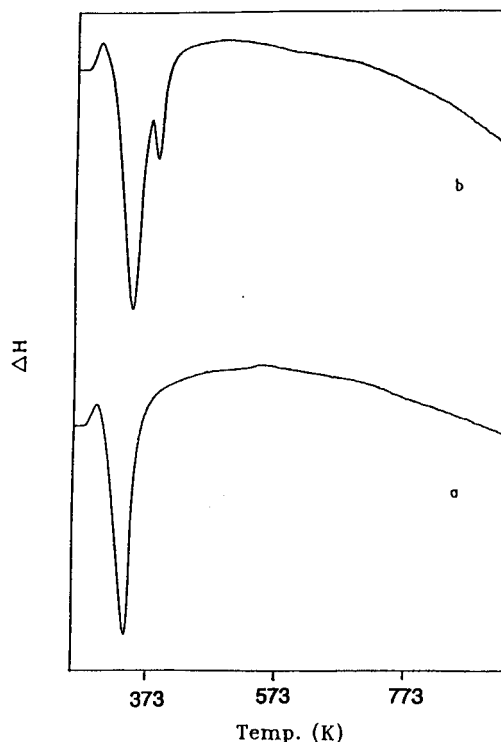
Fig. 4. The DSC thermograms of dealuminated SAPO-11. a: SAPO-11, b: 24h-dealuminated SAPO-11.
