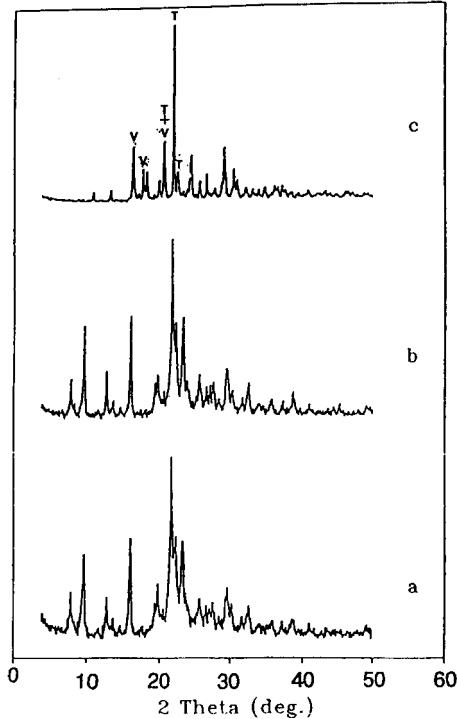
Fig. 1. The X-ray diffractograms of dealuminated SAPO-11. a: SAPO-11, b: 24h-dealuminated SAPO-11, c: 48h-dealuminated SAPO-11, T: tridymite, V: variscite.
