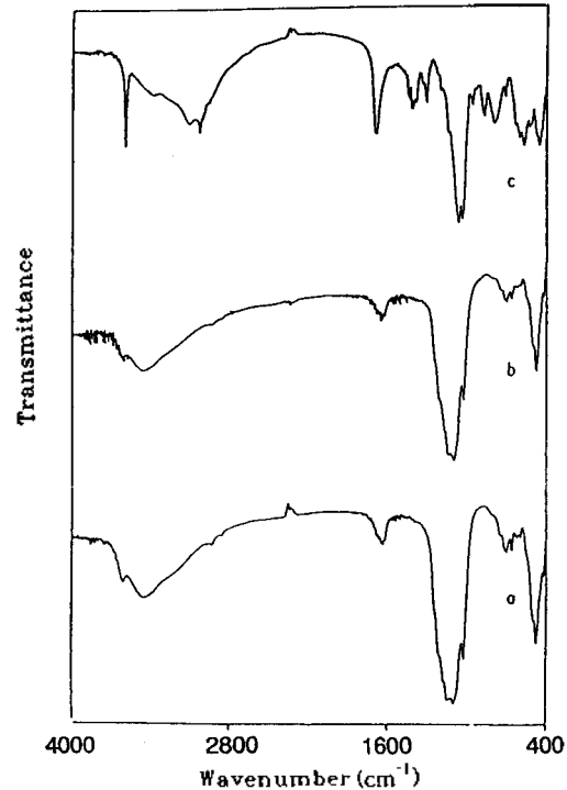
Fig. 2. The IR spectra of dealuminated SAPO-11. a: SAPO-11, b: 24h-dealuminated SAPO-11, c: 48h-dealuminated SAPO-11.
