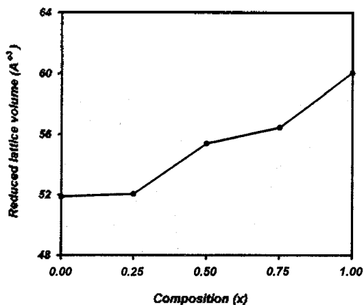
Figure 2. Plot of reduced lattice volume vs x value for the Dy_{1-x}Sr_xCoO_{3-y} system.
