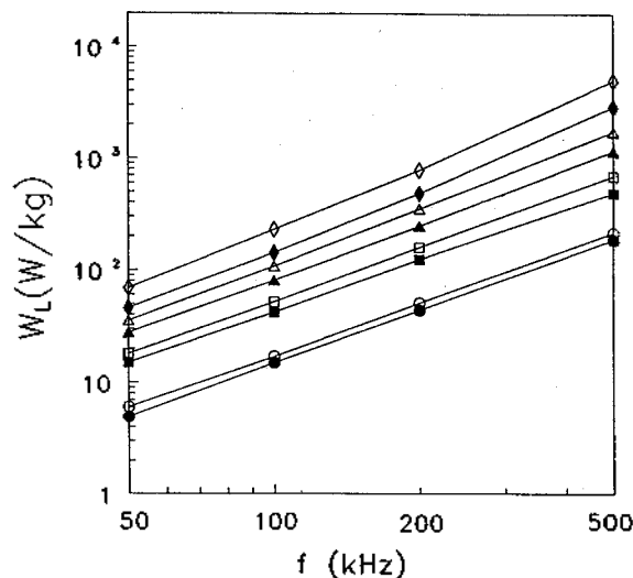
Figure 2. The value of W_L of the Co-based ribbon as a function of frequency ( f ). The results measured at B=0.1, 0.2, 0.3 and 0.4 \text{ T} are indicated by circles, squares, triangles and diamonds, respectively. The uncoated and coated samples are indicated by open and filled symbols, respectively.
