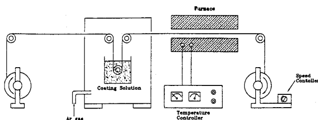
Scheme 1. Schematic diagram of sol-gel dip coating process, showing the sequential stages of dipping and drying at 200 ^\circ\text{C} .
