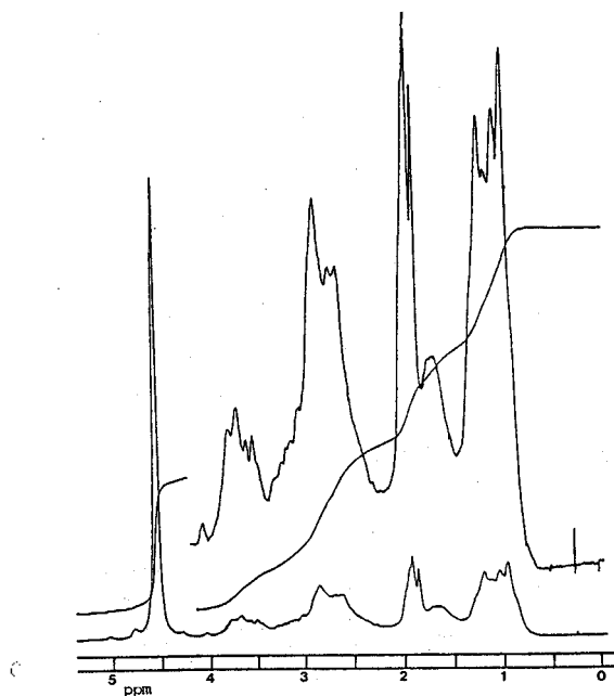
Figure 5. PMR Spectrum of s-cis-mer -[Co(deedba)(L-smc)].
