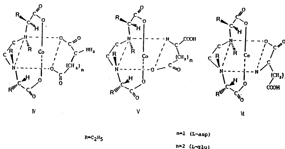
Figure 3. The geometrical isomers of [Co(deedba)(L-aa)] where aa is aspartic or glutamic acid.
