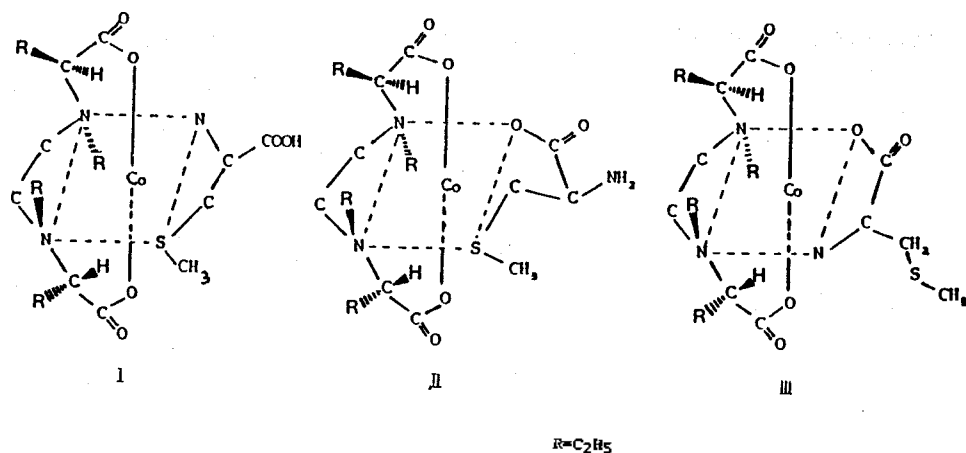
Figure 2. The geometrical isomers of [Co(deedba)(L-smc)] complex.
