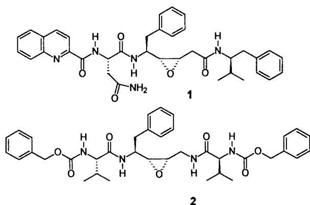
Figure 1. Structures of Irreversible HIV-1 Protease Inhibitors.
