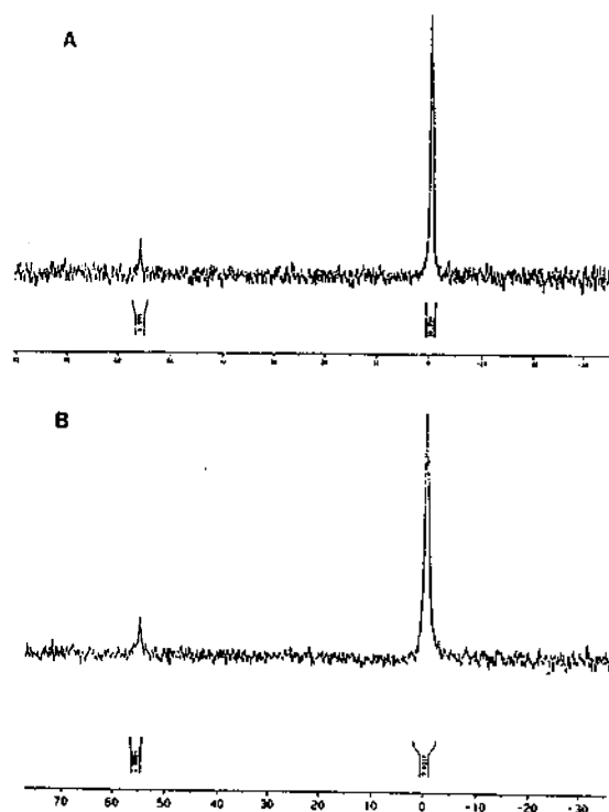
Figure 2. ^{31}\text{P} NMR spectra of the diastereomers of the S_p - and R_p - diastereomers of \text{d}[\text{GATC}_{(p(s))}\text{TCGAGATC}] at 10 °C. The phosphorothioates group of S_p - and R_p - diastereomers resonate at \delta 55.97 and 55.09(B), respectively. Two resonances at \delta -0.29 and 55.97 of the spectrum of R_p isomer(A) and two resonances at \delta -0.12 and 55.09 of the spectrum of S_p isomer (B) were in an approximate ratio of 10 : 1, respectively.
