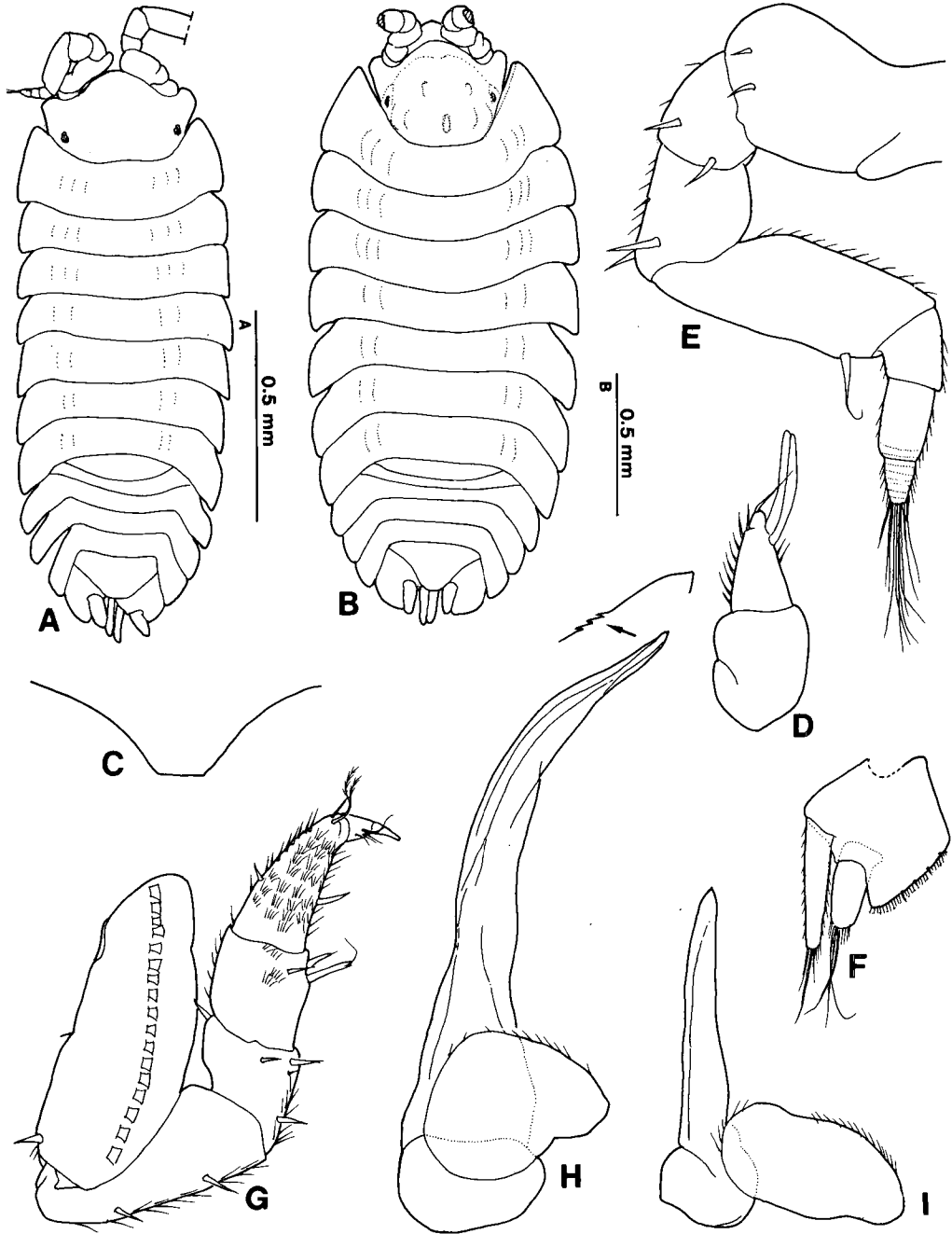
Fig. 3. Armadiilloniscus lanyuensis , n. sp.: A, habitus, male; B, habitus, female; C, telson; D, antennule; E, antenna; F, uropod; G, pereopod 7, male; H, pleopod 1, male; I, pleopod 2, male.
