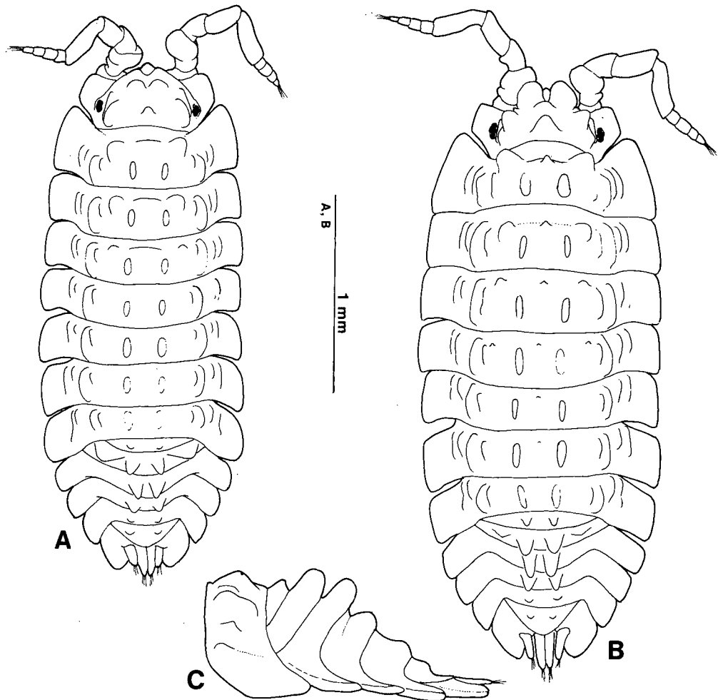
Fig. 1. Armadilloniscus hoonsooi , n. sp.: A, habitus, male; B, habitus, female; C, pereonite 7, pleon and telson, female, lateral view.
