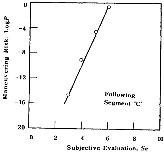
Fig. 14 Maneuvering risk in case of the stern current and wind in segment 'C'
