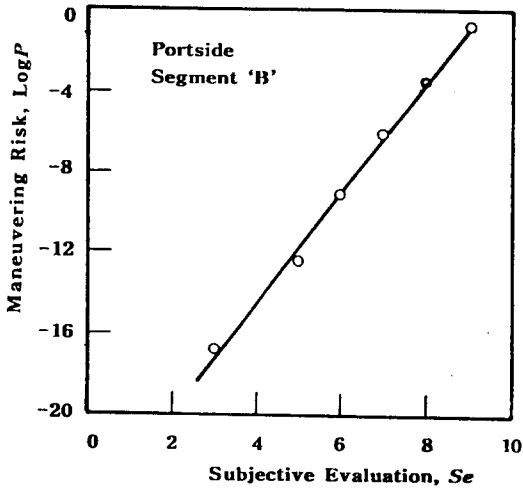
Fig. 7 Maneuvering risk in case of the portside current and wind in segment 'B'
