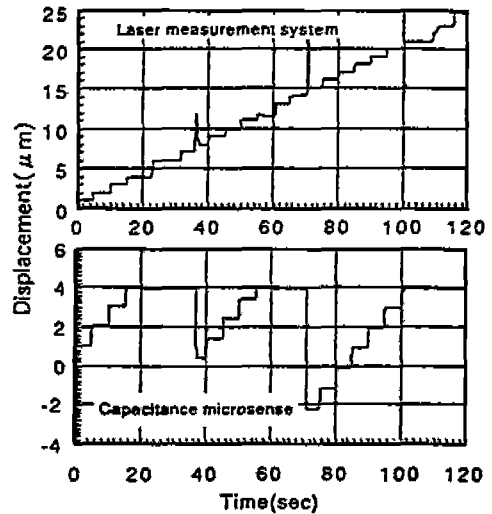
Fig.6 Control of the 1 \mu m Step Positioning
