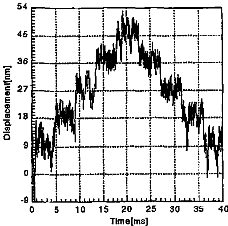
Fig. 8 Resolution for Dual Positioning
