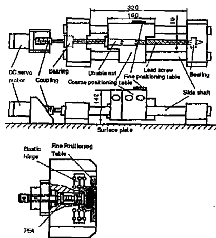
Fig.1 Coarse and Fine Positioning Apparatus
