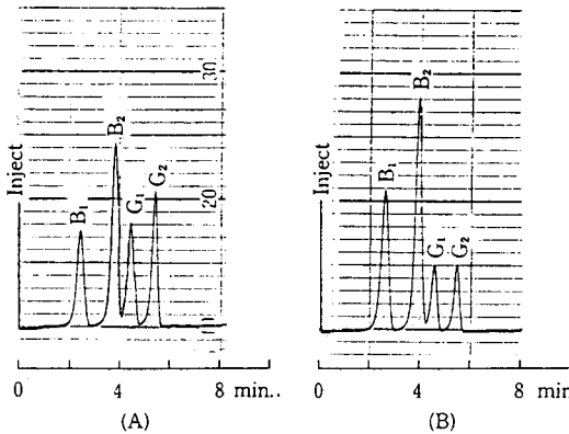
Fig. 7 HPLC chromatogram of same standard solution at Em 350/Ex 420 and Em 360/Ex 445 nm of fluorescence detector.
