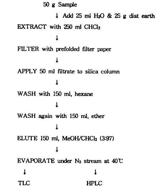
Fig. 1. Extraction of Aflatoxins by AOAC-CB method.
