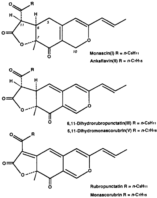
Fig. 3. Chemical structures of Monascus yellow and red pigments.
