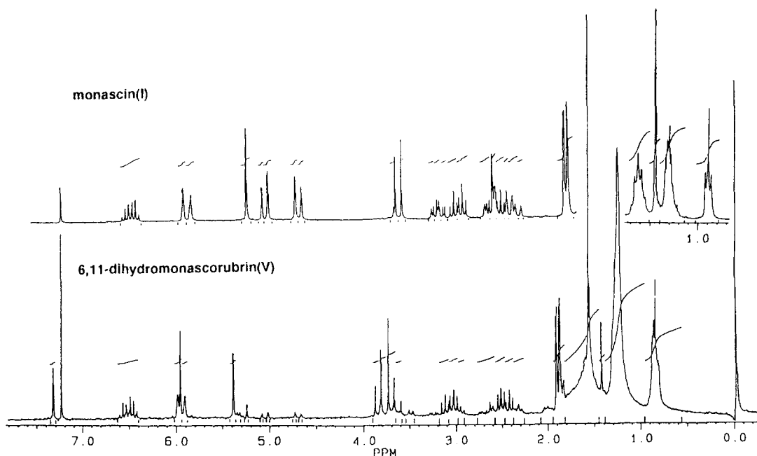
Fig. 2. H^1 NMR spectrum of monascin(I) and 6,11-dihydromonascorubin(V).
