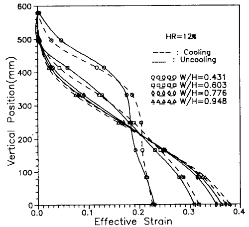
Fig. 8 Effect of die width ratio on equivalent strain distribution in vertical direction
