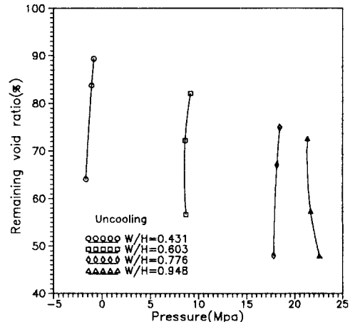
Fig. 13 Relation between pressure and remaining void area ratio in uncooled case
