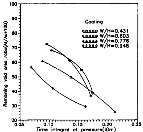
Fig. 17 Relation between time integral of pressure and remaining void area ratio in cooled case
