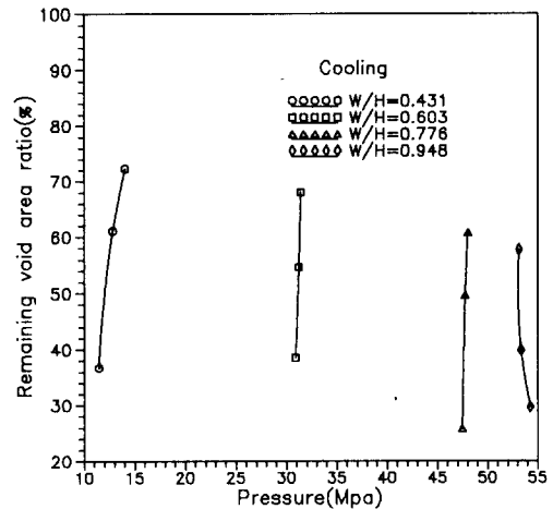
Fig. 16 Relation between pressure and remaining void area ratio in cooled case
