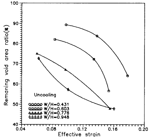
Fig. 12 Relation between reduction of height and remaining void area ratio in uncooled case
