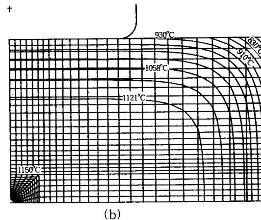
Fig. 2 Initial mesh(a) and initial temperature distribution(b) after 45 minute pre-cooling
