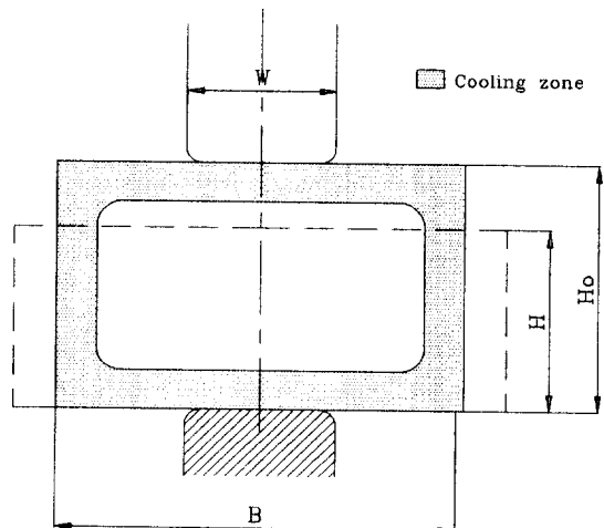
Fig. 1 Schematic diagram of the analysis model
