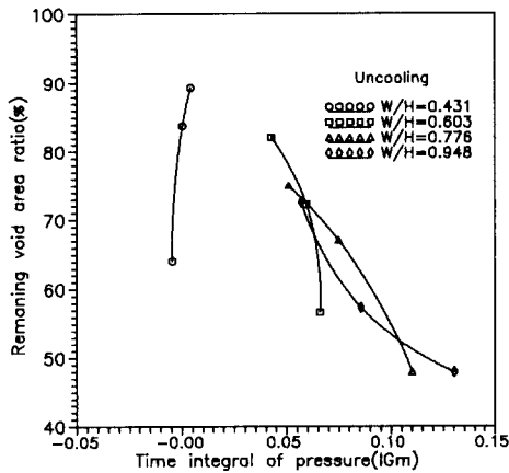
Fig. 14 Relation between time integral of pressure and remaining void area ratio in uncooled case
