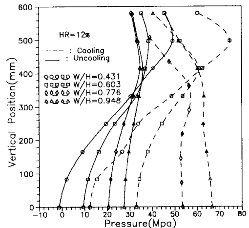
Fig. 9 Effect of die width ratio on pressure distribution in vertical direction
