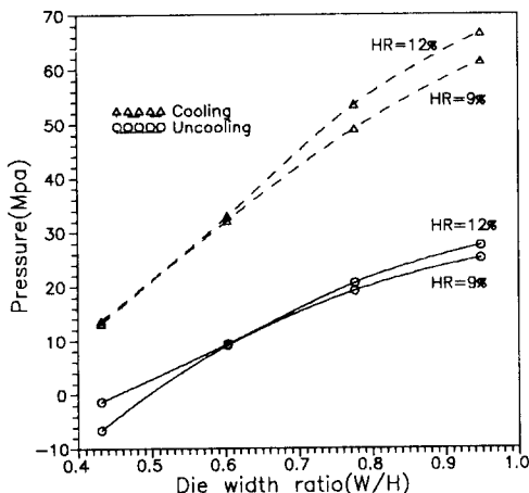
Fig. 7 Relation between die width ratio and pressure in case of uncooling and cooling
