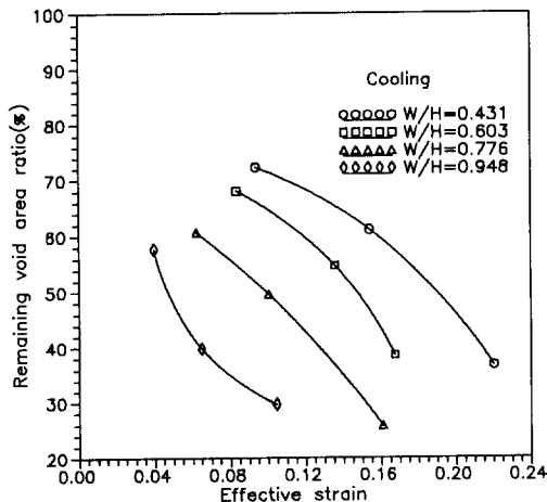
Fig. 15 Relation between reduction of height and remaining void area ratio in cooled case
