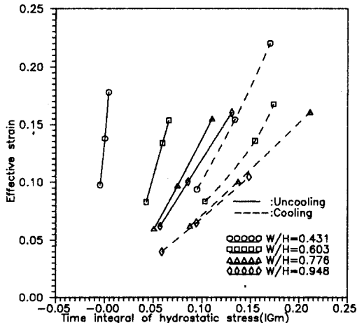
Fig. 18 Relation between time integral of hydrostatic stress and remaining void area ratios
