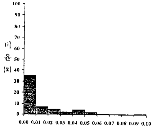
(Fig. 1) Differences between the Basic Lexical Probability Estimation Formula and the 1st Order Approximate Lexical Probability Estimation Formula
