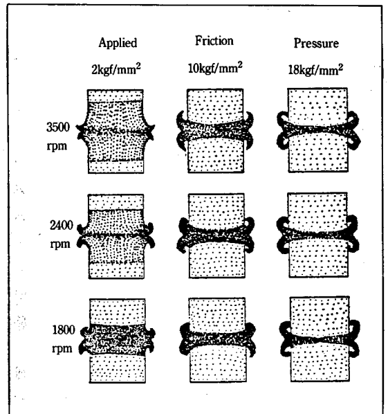
Fig. 4. Variation of the heat affected zone with rotation speed and applied pressure in the fixed pressure brake method.(S25C, Specimen dia.=18mm, Friction distance =5.5mm)
