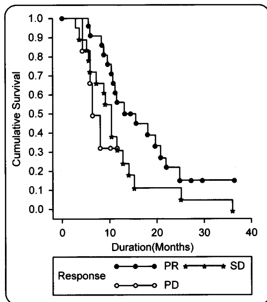
Fig. 4 Advanced NSCLC Kaplan-Meier survival plot by Response(p=0.056)
