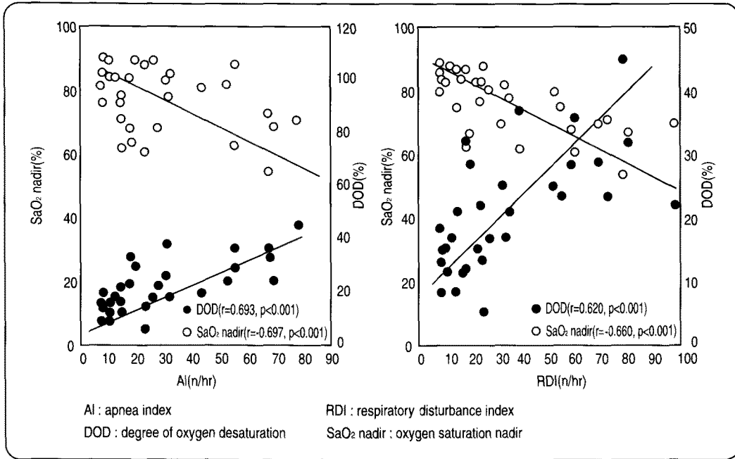
Fig. 2. Correlations of apnea index, respiratory disturbance index, oxygen saturation nadir and degree of oxygen desaturation.
