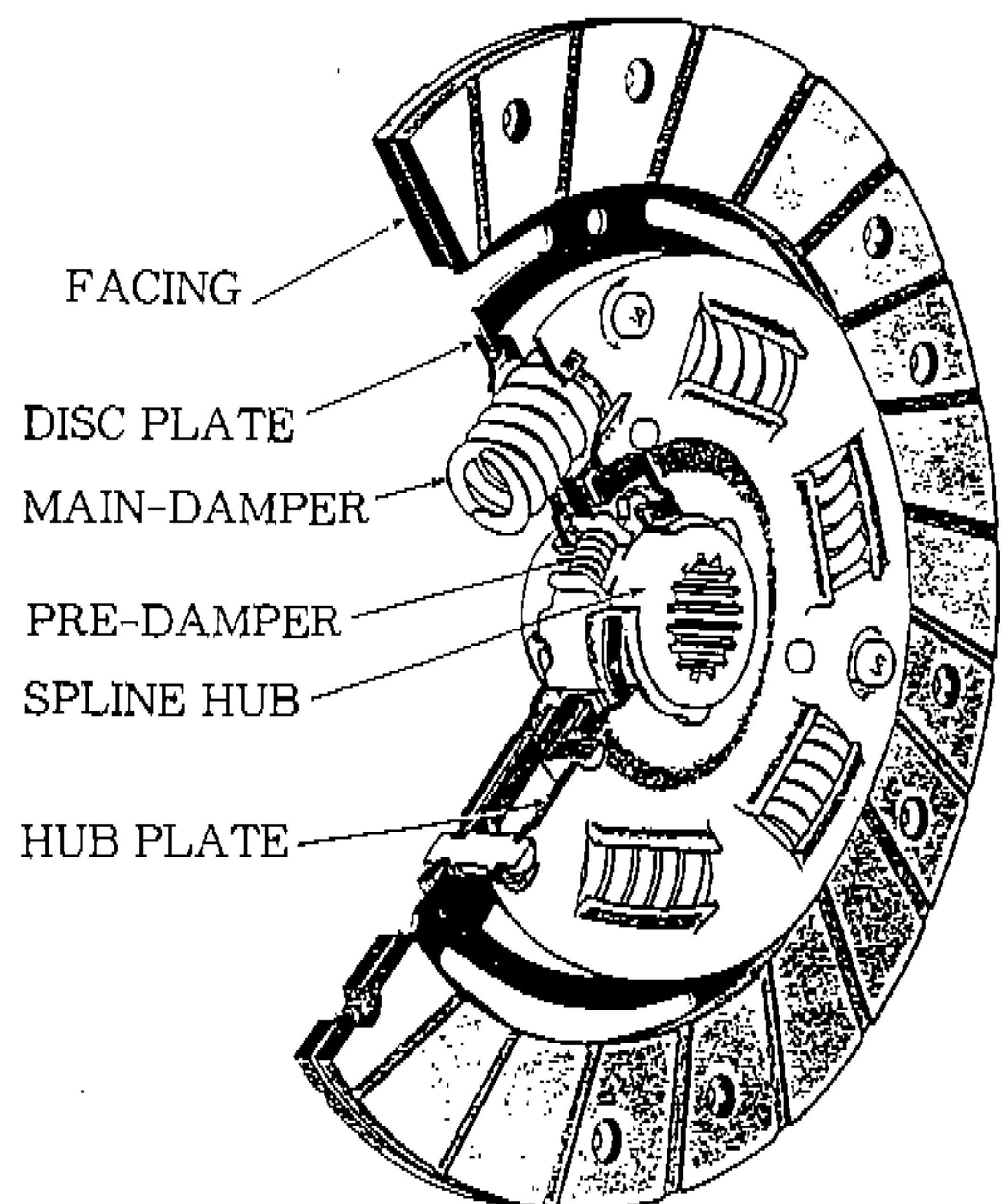
Fig.1 Clutch disc assembly
