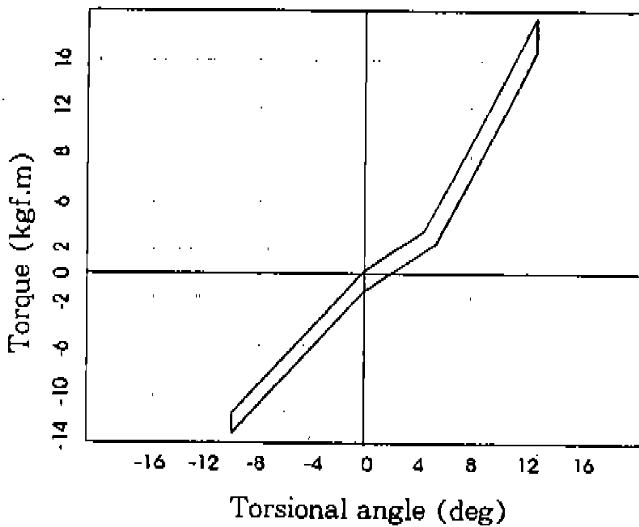
(b) x21 clutch
