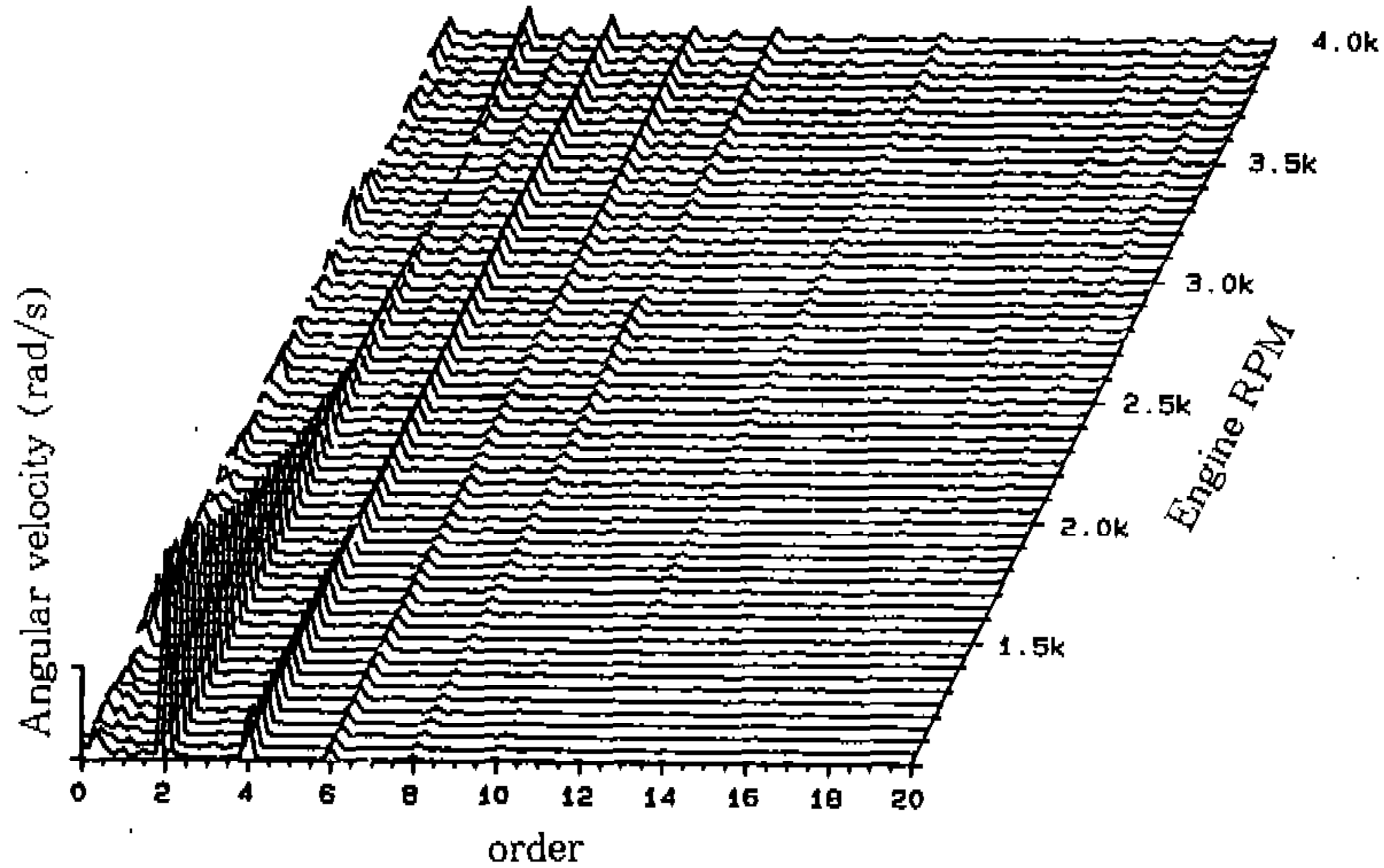
Fig.6 Angular velocity in engine-flywheel at driving
