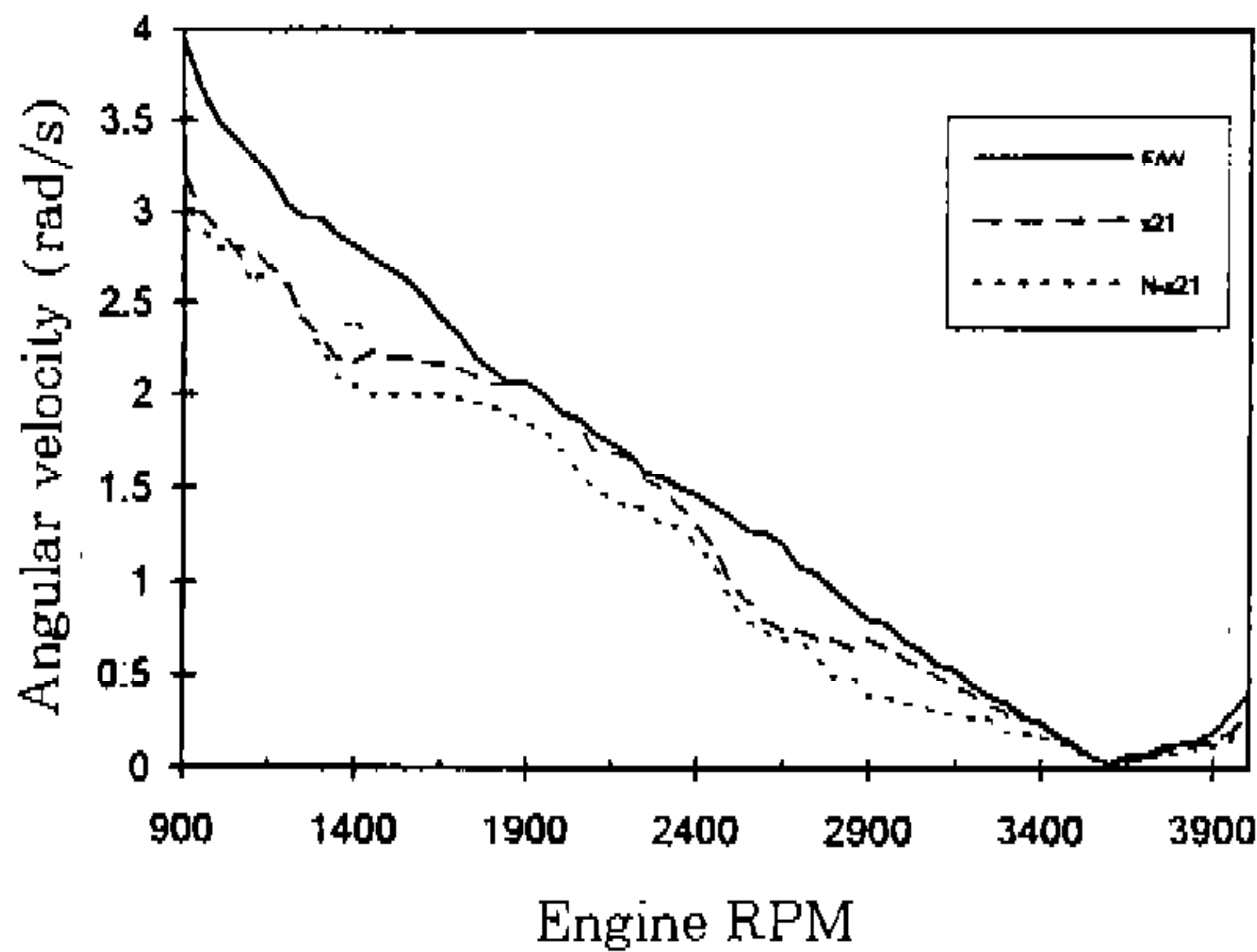
(a) 3rd gear driving
