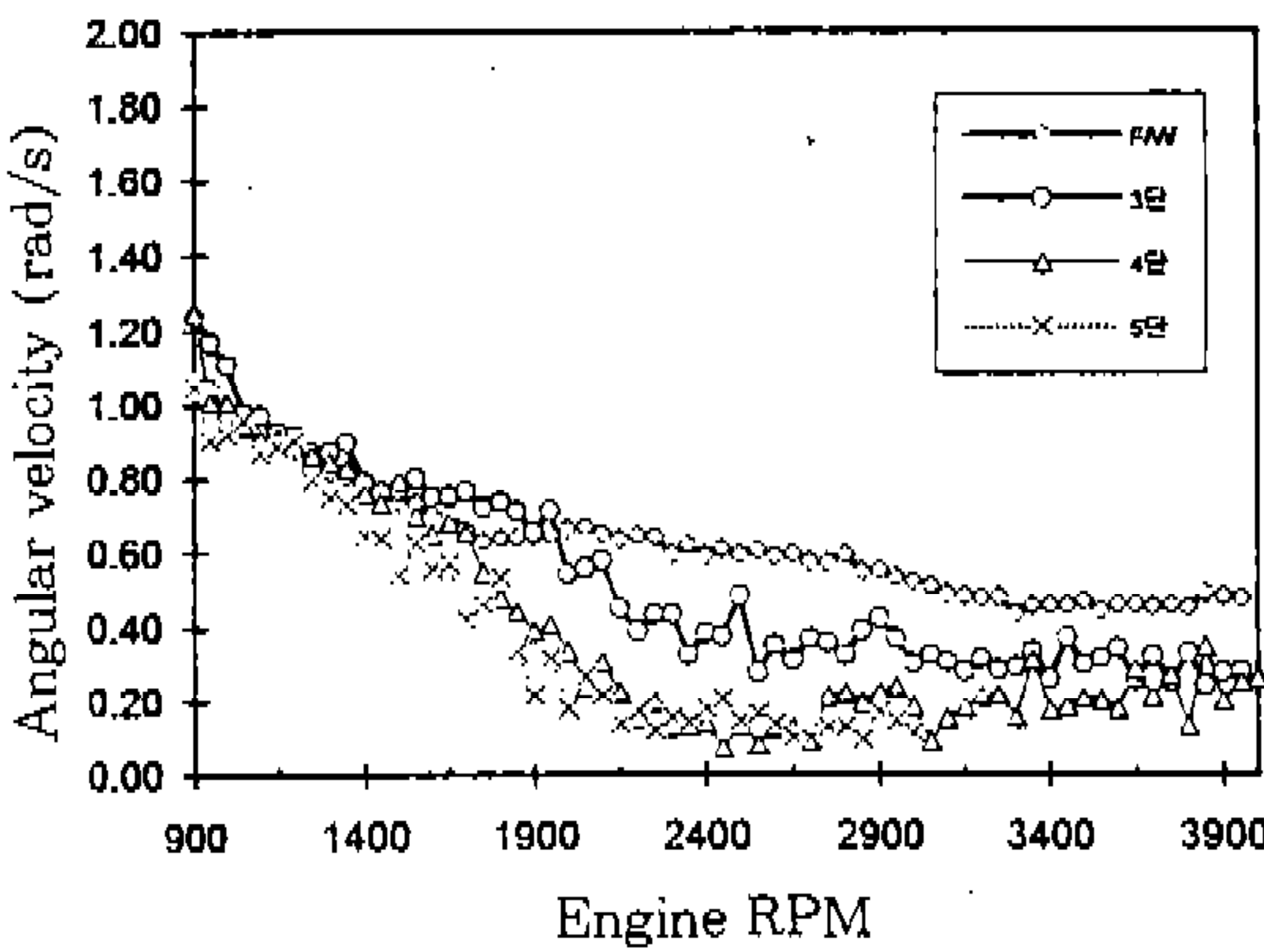
(b) x21 clutch
