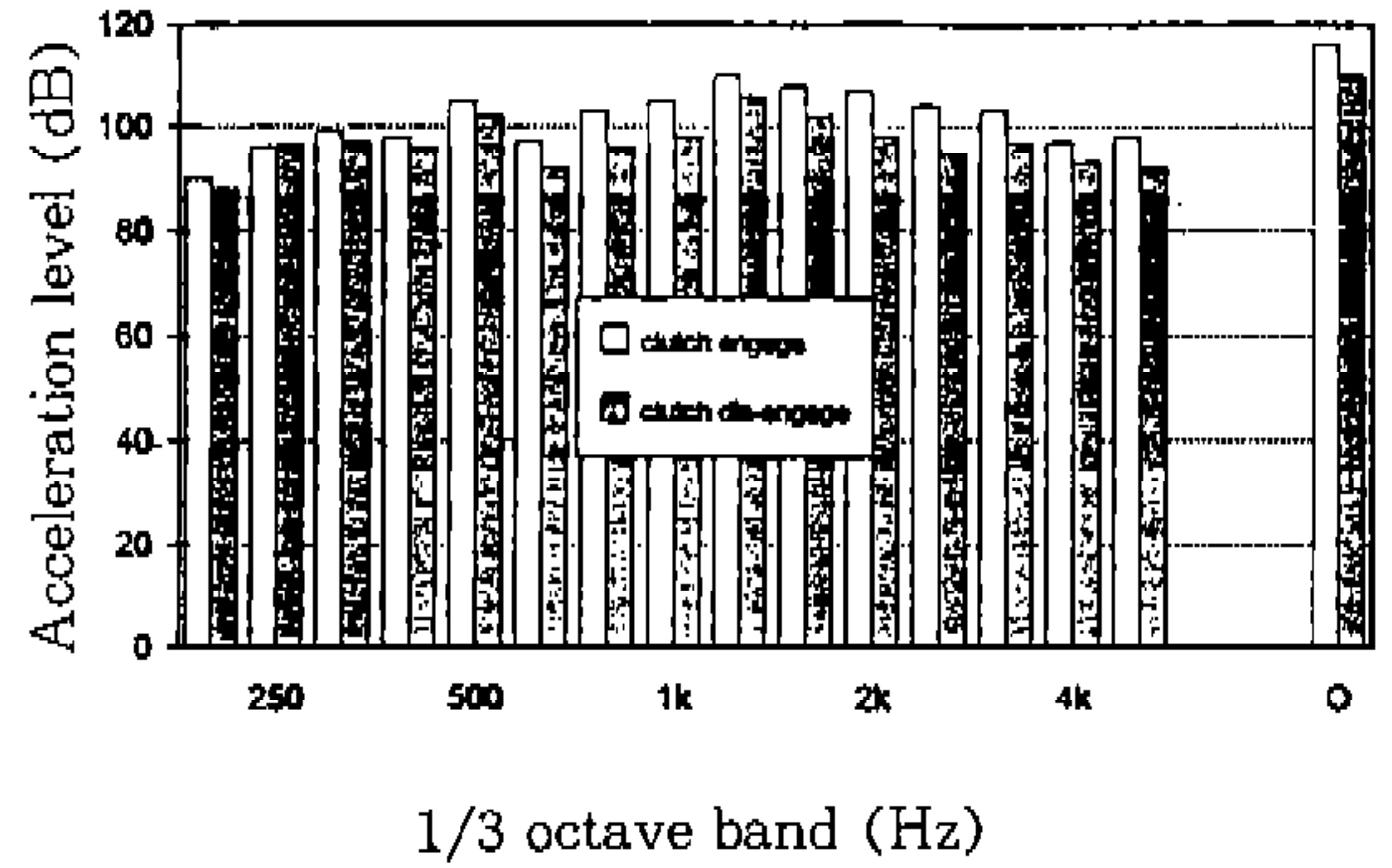
(a) x11 clutch
