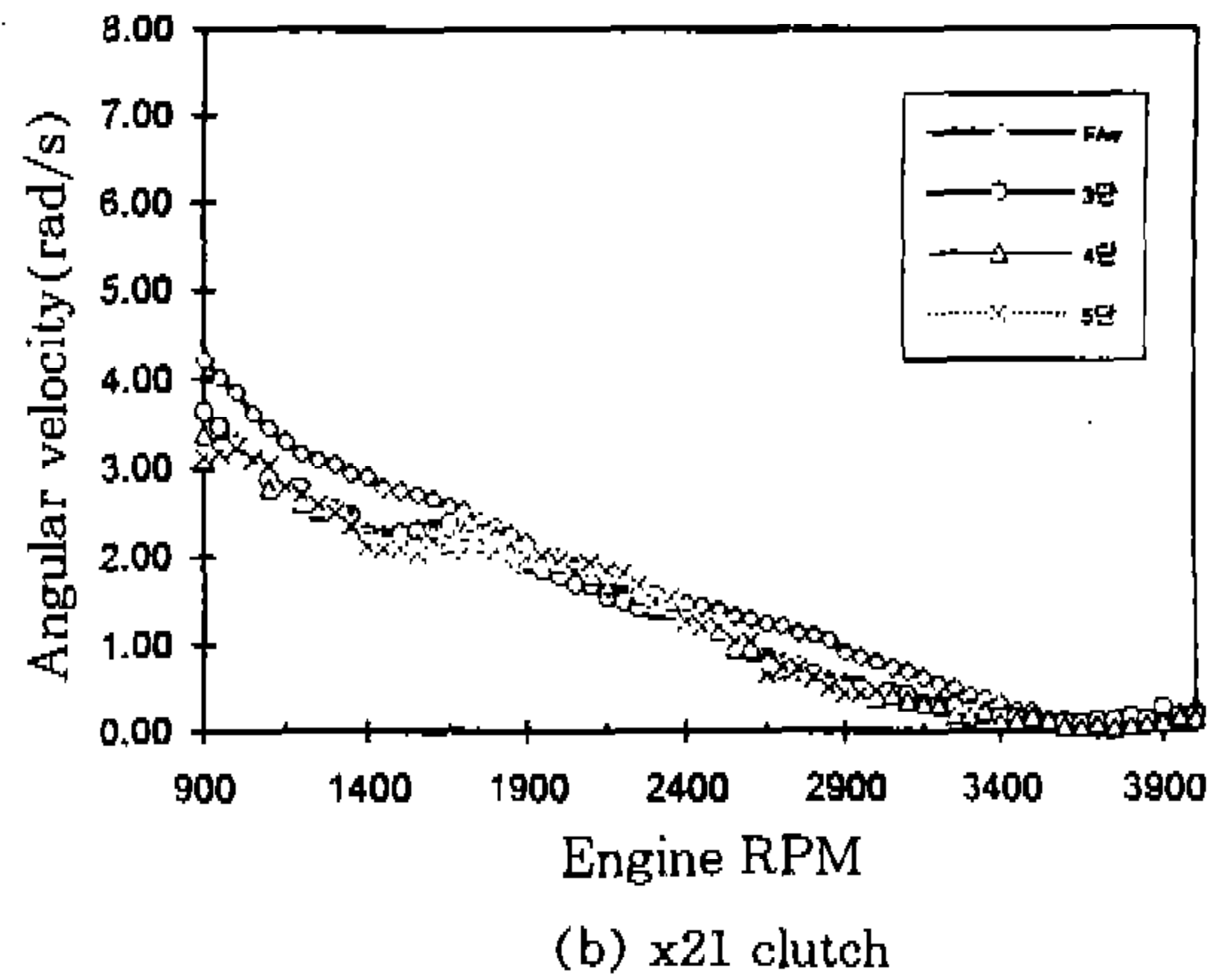
Fig.7 Angular velocity of second order in engine flywheel and input gear at driving.
