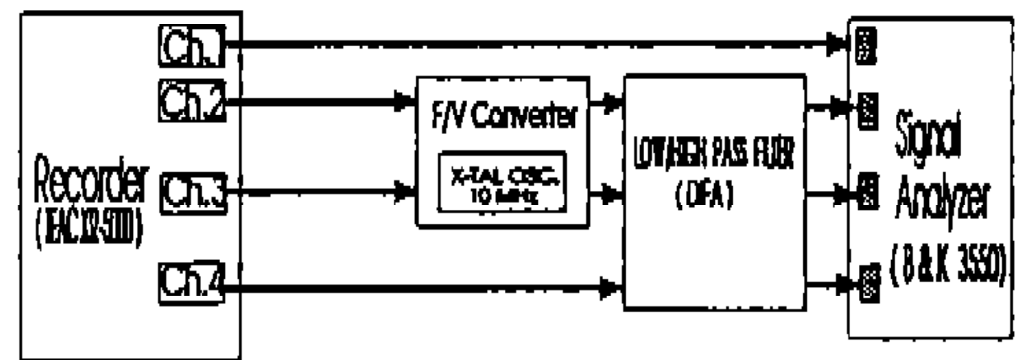
(b) the analysing Instrument system
