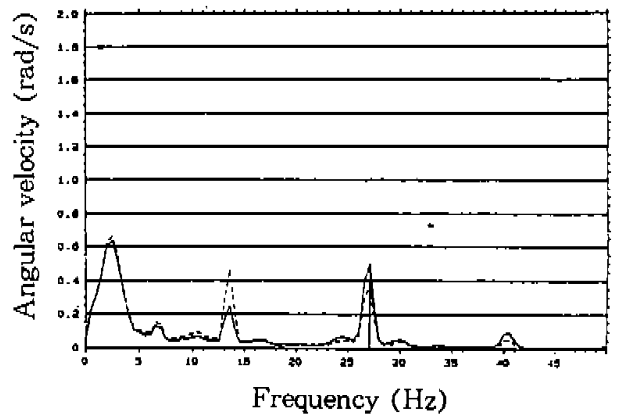
(b) N-x21 clutch
