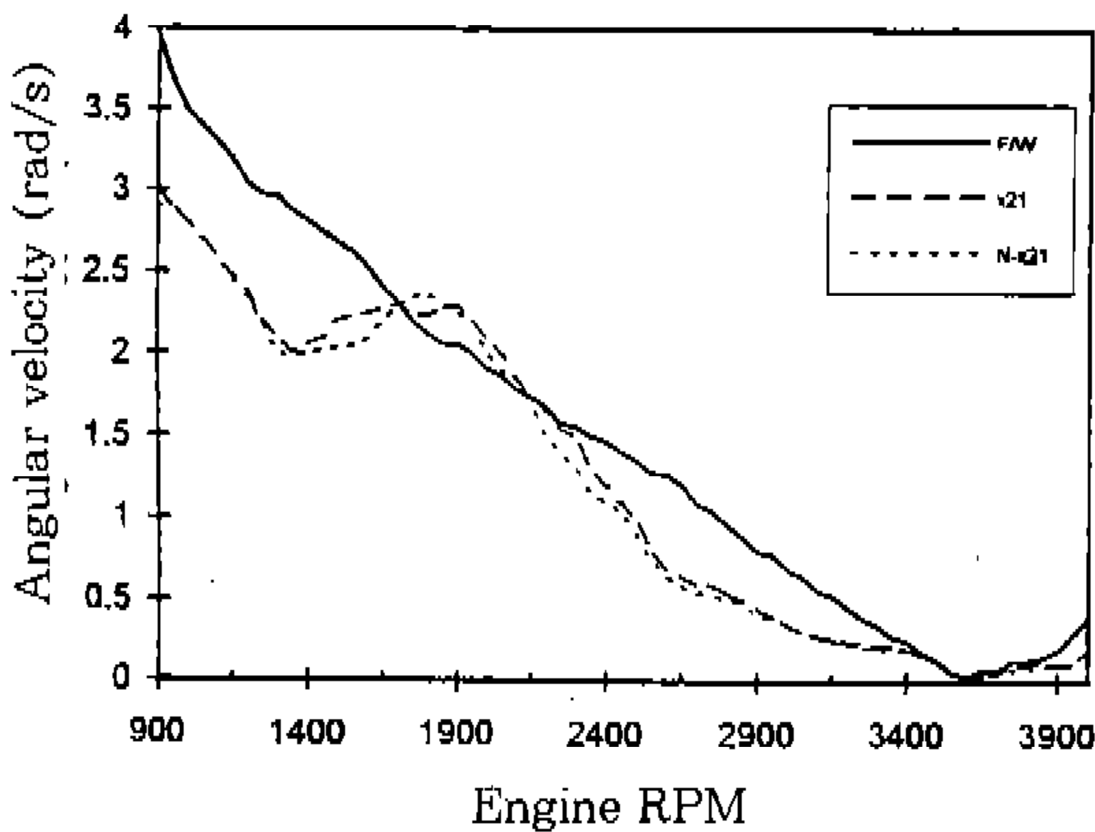
(b) 4th gear driving
