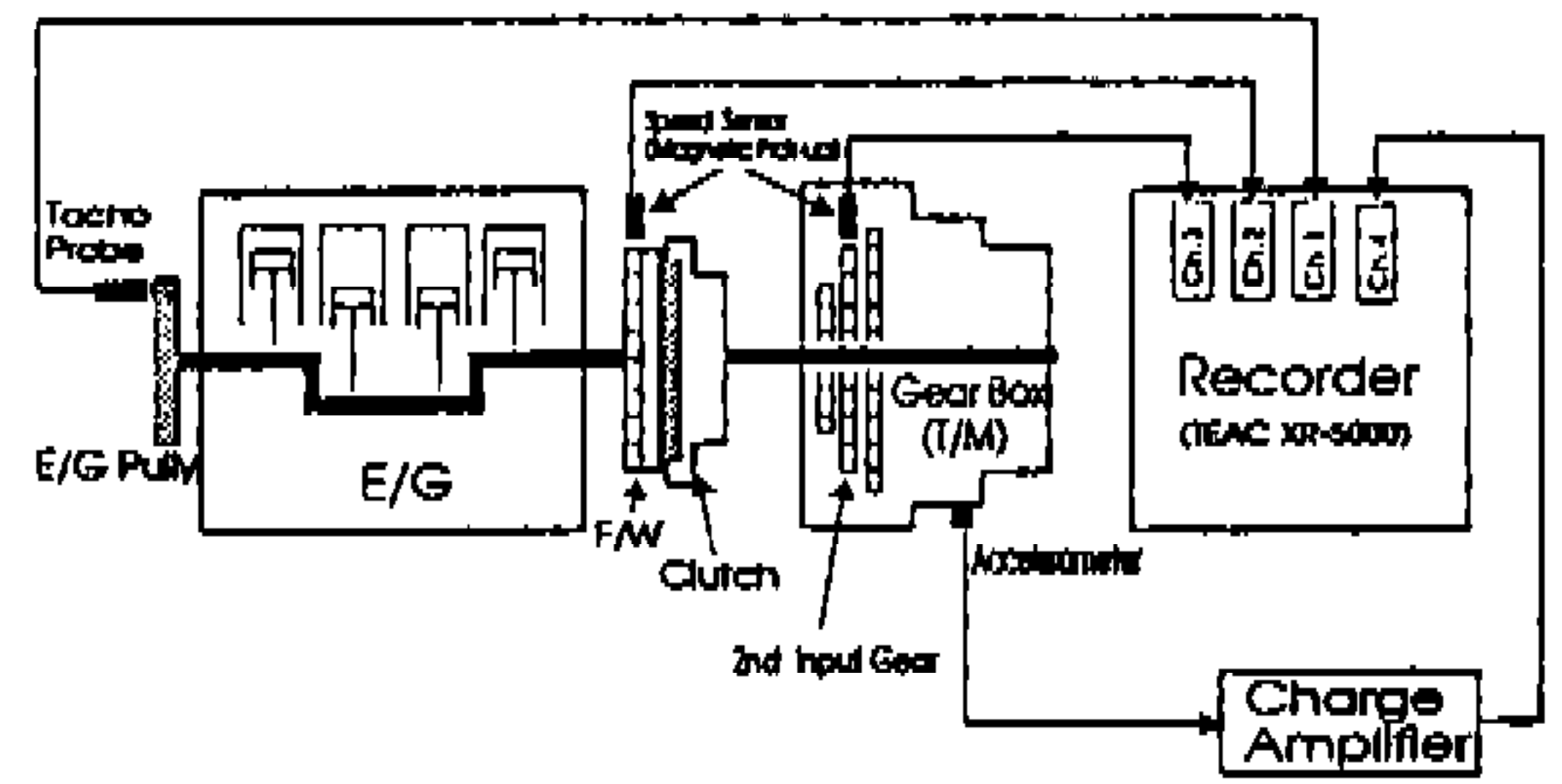
(a) the measuring Instrument system
