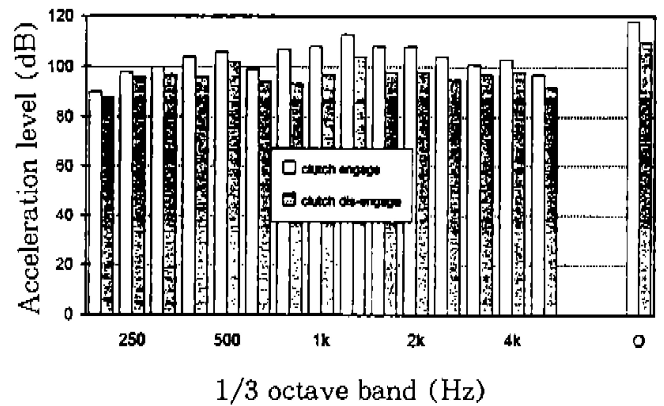
(b) x21 clutch
