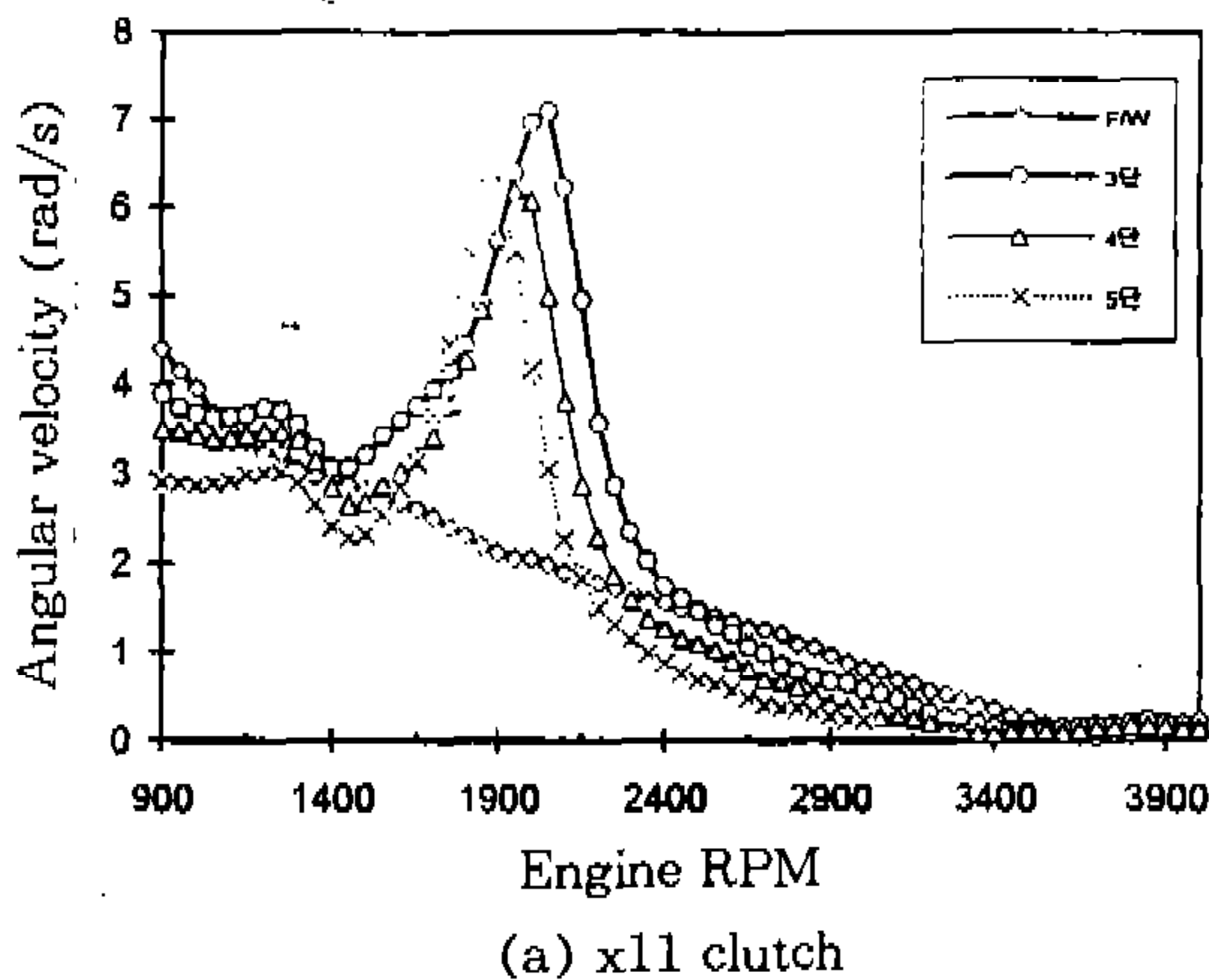
Fig.7 Angular velocity of second order in engine flywheel and input gear at driving.
