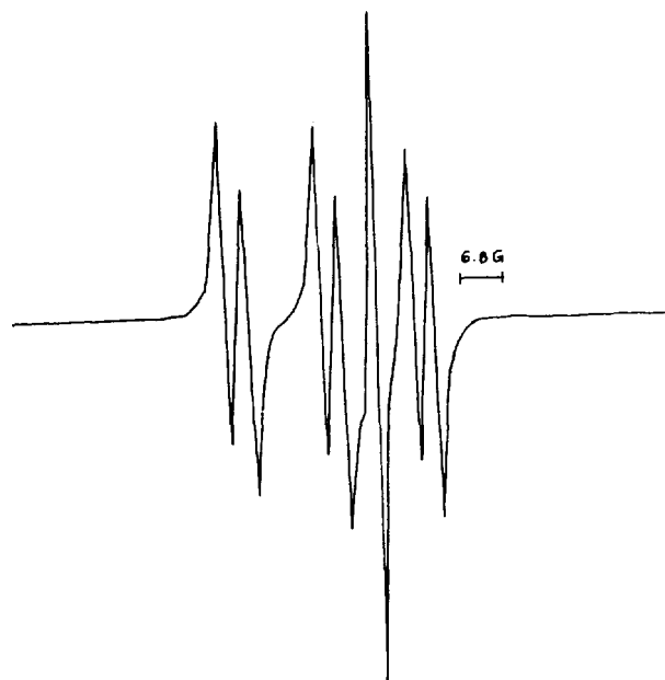
Figure 1. ESR spectrum of the PBNEt radical formed in the reaction of ethyl bromide with Li (1% wt. Na) in DBE at r.t. (scanned in 5 min. after mixing).
