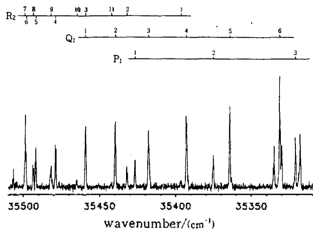
Figure 1. Portion of the LIF spectra of OH produced from photodissociation of \text{H}_2\text{O}_2 employing the v=1\leftarrow 0 , {}^2\Sigma\leftarrow {}^2\Pi electronic transition. Assignments of the rotational transitions are on top of the peaks.
