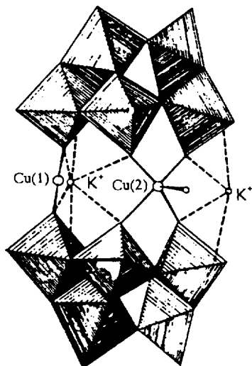
Figure 1. The structure of [\text{As}_2\text{W}_{18}\text{O}_{66}\text{Cu}_3(\text{H}_2\text{O})_2]^{12-} (reproduced from ref 4).
