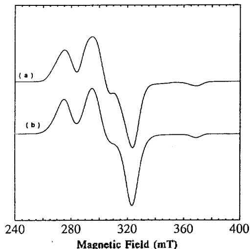
Figure 7. (a) Experimental and (b) calculated powder EPR spectrum of K_{12}[As_7W_{18}O_{66}Cu_3(H_2O)_2] \cdot 11H_2O at 77 K.
