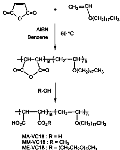
Scheme 2. Preparation scheme of the copolymers, MA-VC18, MM-VC18, and ME-VC18.
