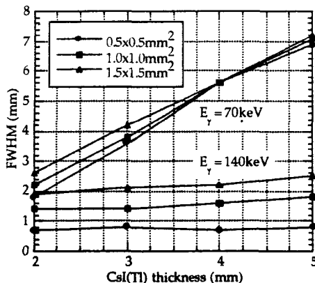
Fig. 5 Intrinsic resolution of a-Si : H based gamma camera as a function of CsI(Tl) thickness with different pixel size.
