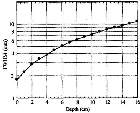
Fig. 3 Spatial resolution (FWHM) as a function of depth (source-to-collimator distance) for Picker low-energy-high-resolution, parallel-hole collimator.
