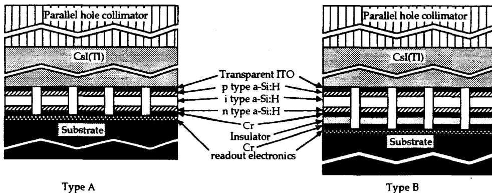
Fig.1 Cross sectional diagram of two a-Si : H based gamma cameras. 5 pixels are drawn for each type. Type A has a conventional p-i-n a-Si : H photodiode array and can be operated either in event-by-event collection mode or interaration mode. Type B has additional storage capacitors(Cr-insulator-Cr layers) coupled to p-i-n a-Si : H photodiodes and it can be operated only in integration mode. See text for details.
