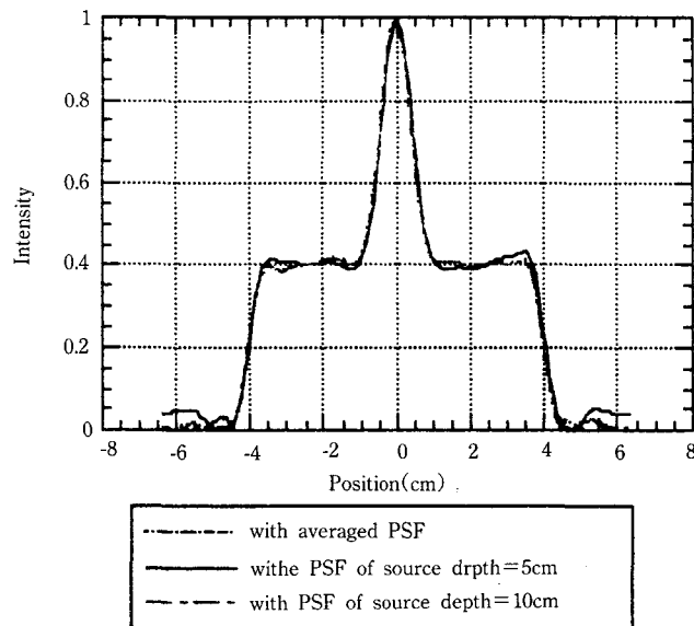
Fig. 11 X-directional profile of restored images using different PSF. Although PSFs are different depending on the source depth, the resultant images are not sensitive to the mismatch in the PSF.
