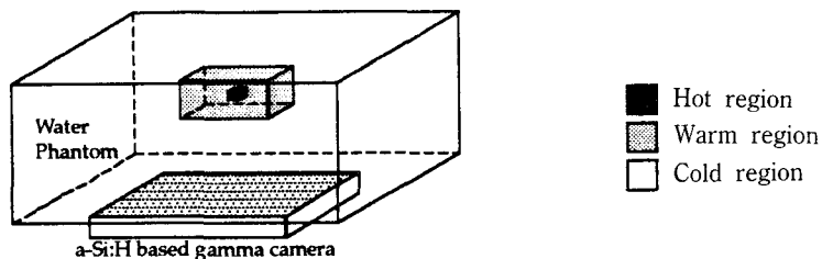
Fig. 6 The geometry of the water phantom with hot, warm and cold sources
