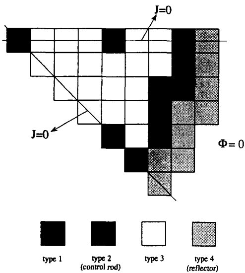
Fig. 1. Configuration of the IAEA-2D Benchmark Problem
