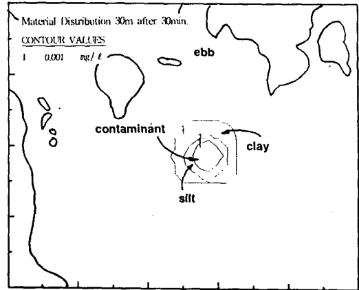
Fig. 5.5 Material distribution for 30m water depth(ebb flow)
