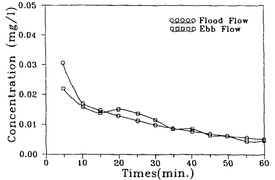
Fig. 5.2 Change of peak contaminant concentration in water column with respect to time
