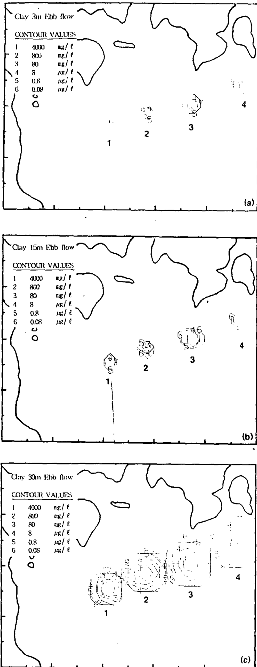
Fig. 5.4 Material distribution for the selected water depth(ebb flow, clay) : (a) 3m,(b) 15m,(c) 30m
