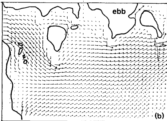
Fig. 4.1 Model boundary and applied flows : (a) flood flow, (b) ebb flow
