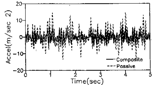
(b) Passive and composite suspension
