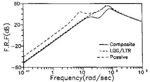
Fig. 7 Acceleration frequency response functions for composite, LQG/LTR and passive suspension
