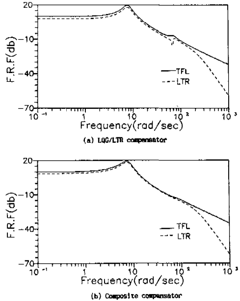
Fig. 4 Singular values of the loop TFM
