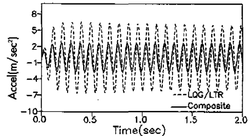
Fig. 12 Acceleration responses of the sprung mass for the sinusoidal input of 67.3 \text{ rad/sec}
