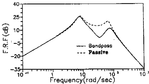
Fig. 6 Velocity frequency response functions for bandpass feedback active and passive suspension
