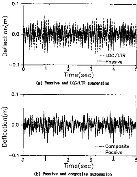
Fig. 10 Tire deflections
