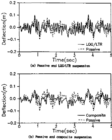
Fig. 9 Suspension deflections
