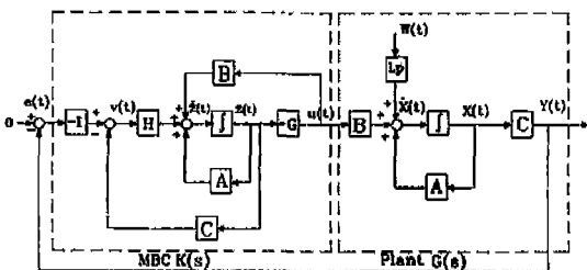
Fig. 3 Output feedback control system
