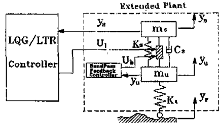
Fig. 1 Active suspension system with composite controller
