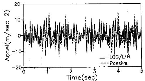
(a) Passive and LQG/LTR suspension
