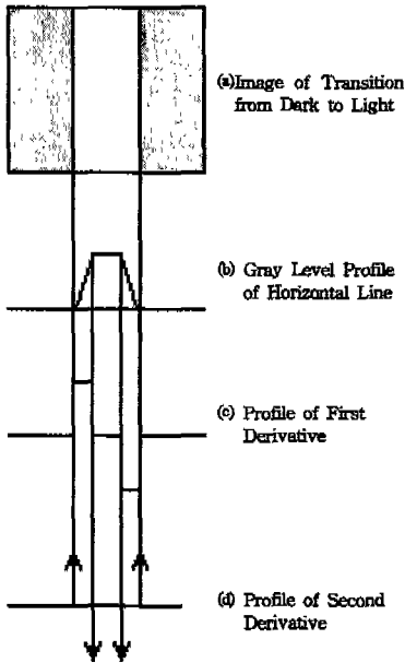
Fig. 3 Elements of edge detection by derivative operators
