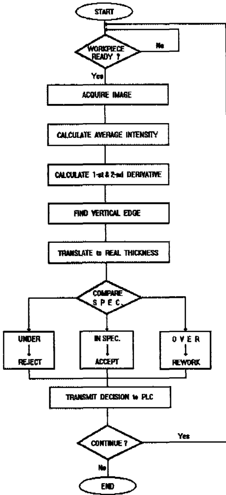
Fig. 7 Orders for acquirement of image and decision
