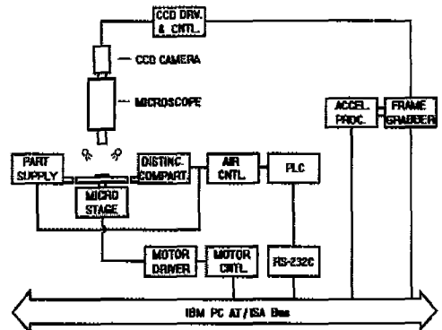
Fig. 5 Block diagram of automatic thickness measuring system
