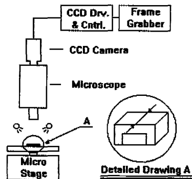
Fig. 1 Working principle of automatic thickness measuring system
