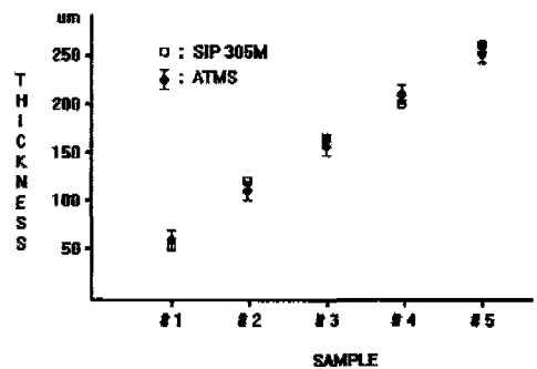
Fig. 16 Graph of the ATMS vs. the SIP 305M
