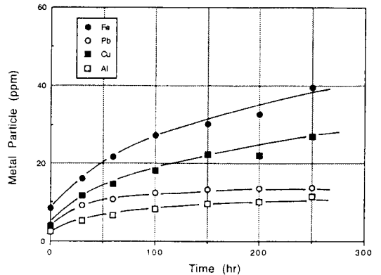
Fig. 8. Concentration of metal particles in used oil from the cultivator engine.
