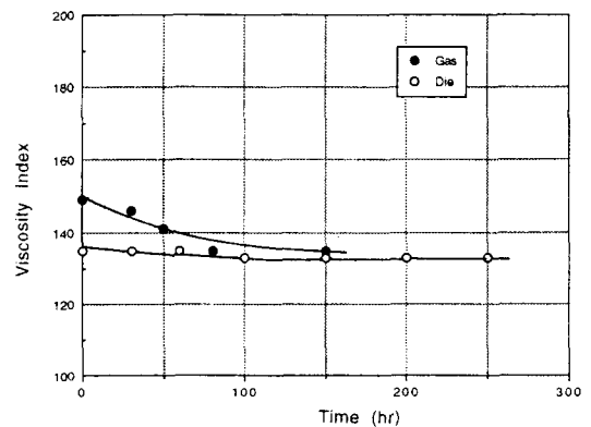
Fig. 3. Change of viscosity index of used oil.
