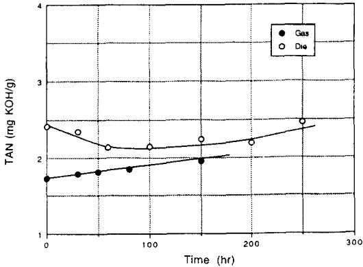
Fig. 4. Change of TAN in used oil.
