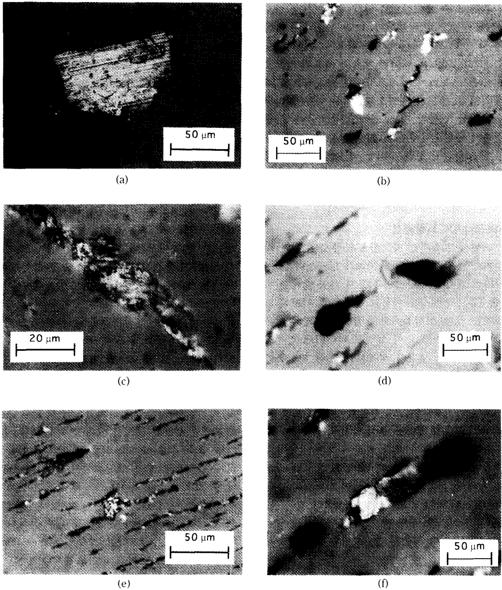
Fig. 9. Wear particles in used oil. (a) Severe wear particle (b) Cutting wear particle (c) Temper colored wear particle (d) Dark metallo Oxide (e) Particle chunk with sphere particle (f) Polarized severe wear particle.
