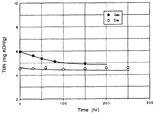
Fig. 5. Change of TBN in used oil.
