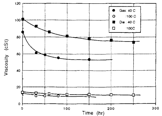
Fig. 2. Change of kinematic viscosity of used oil.
