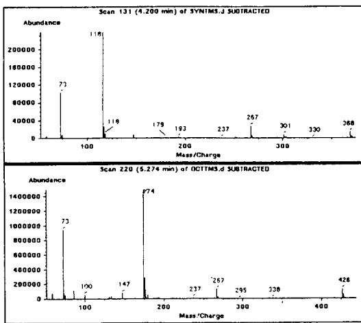
Fig. 1. Mass spectra of synephrine-(O-TMS) 2 -N-TMS and octopamine-(O-TMS) 2 -N-TMS.
