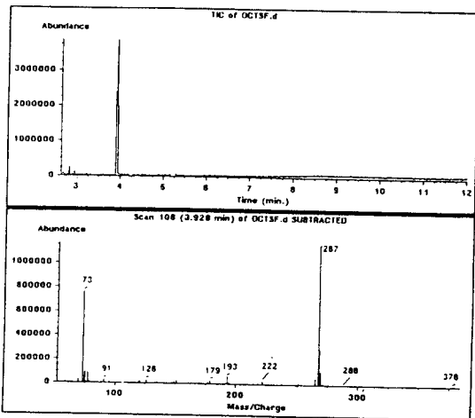
Fig.4. Total ion chromatogram and mass spectrum of octopamine-(O-TMS) 2 -N-TFA.
