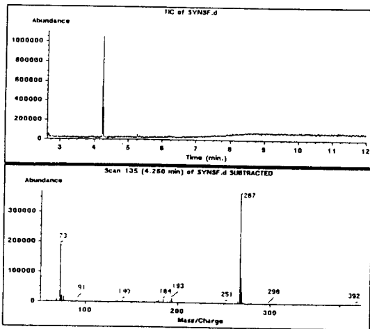
Fig. 3. Total ion chromatogram and mass spectrum of synephrine-(O-TMS) 2 -N-TFA.
