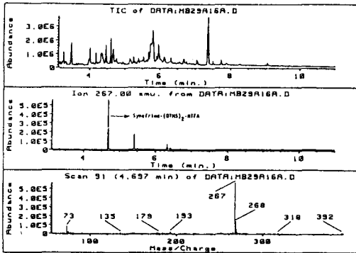
Fig. 8. Total ion chromatogram and ion chromatogram of the derivatized urinary extract of a volunteer who has taken 5 cans of the sample D-1 and mass spectrum of synephrine-(O-TMS) 2 -N-TFA.
