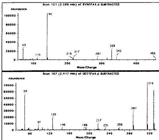
Fig. 2. Mass spectra of synephrine-(O-TFA) 2 -N-TFA and octopamine-(O-TFA) 2 -N-TFA.
