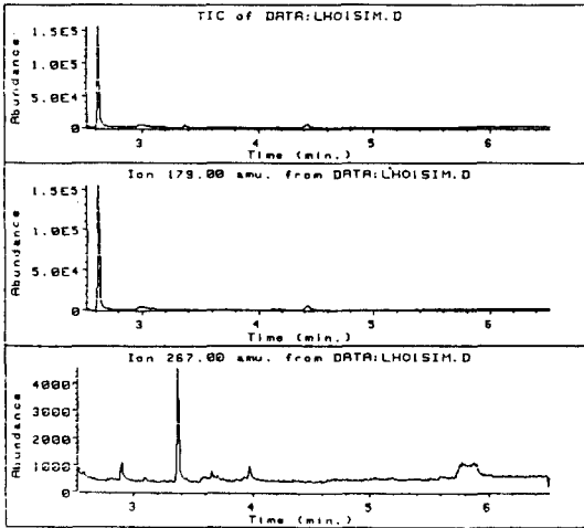
Fig. 7. Total ion chromatogram and ion chromatogram of the blank urinary extract.
