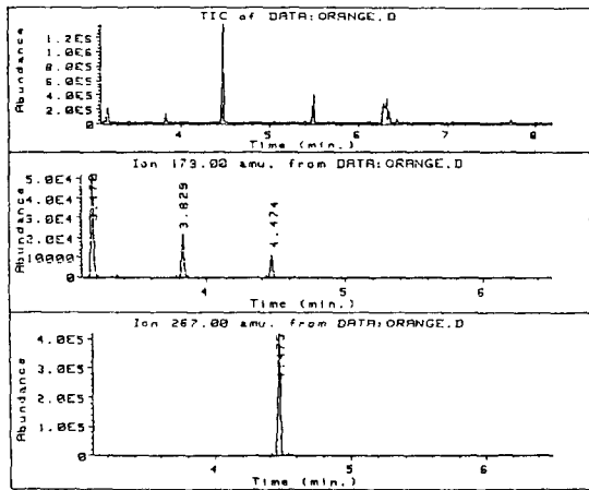
Fig. 5. Total ion chromatogram and ion chromatogram of the derivatized ether extract of the sample D-1.
