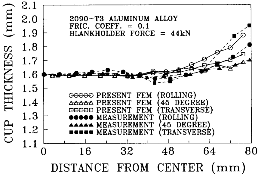
Fig. 4 Comparison of predicted and measured thickness distribution for the Al2090 cup drawing simulation
