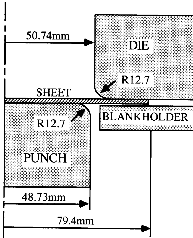
Fig. 1 Tooling geometry for cylindrical cup drawing operation
