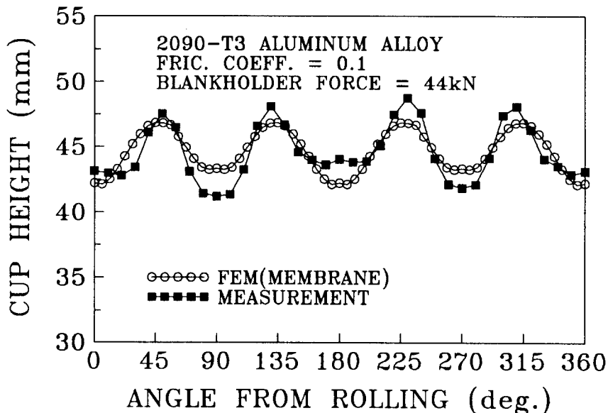
Fig. 3 Comparison of predicted and measured cup heights and earing profiles for the Al2090 cup drawing test
