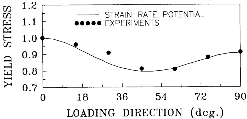
Fig. 5 Normalized yield stress anisotropy measured and predicted with the Barlat's strain-rate potential
