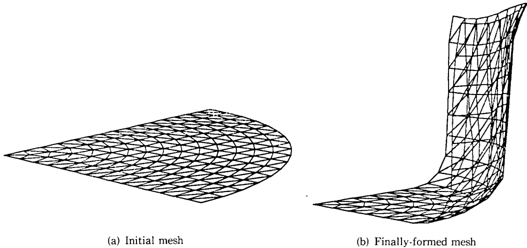
Fig. 2 (a) Initial FEM mesh and (b) finally-formed one for simulating a cylindrical cup drawing operation
