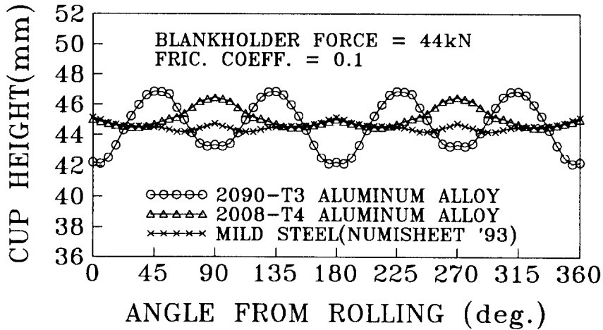
Fig. 7 Comparison of predicted cup heights and earing profiles with the present FEM(AI2090, AI2008 & mild steel)
