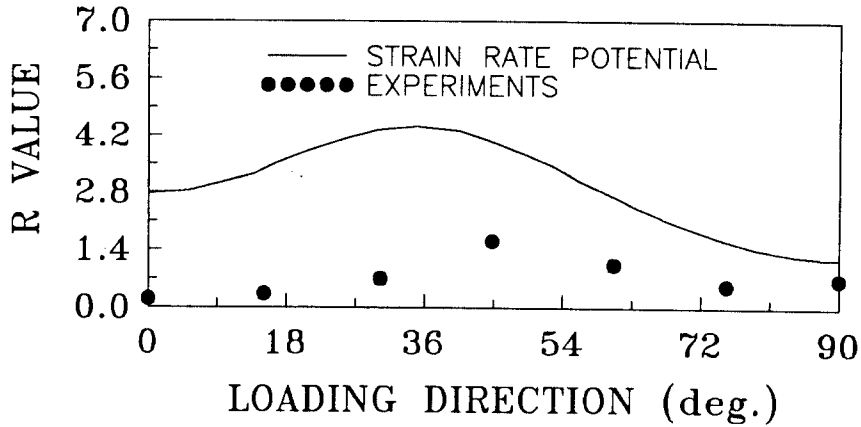
Fig. 6 R(Lankford) value anisotropy measured and predicted with the Barlat's strain-rate potential
