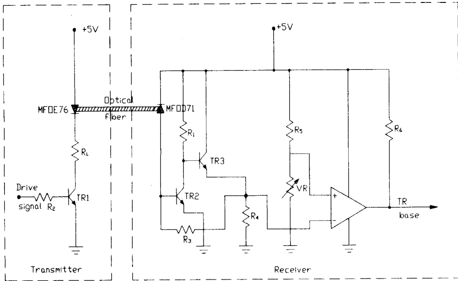
Fig. 8 Transmitter and receiver circuits of Optical transmission system
