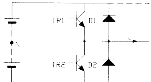
Fig. 5 One phase circuit of inverter
