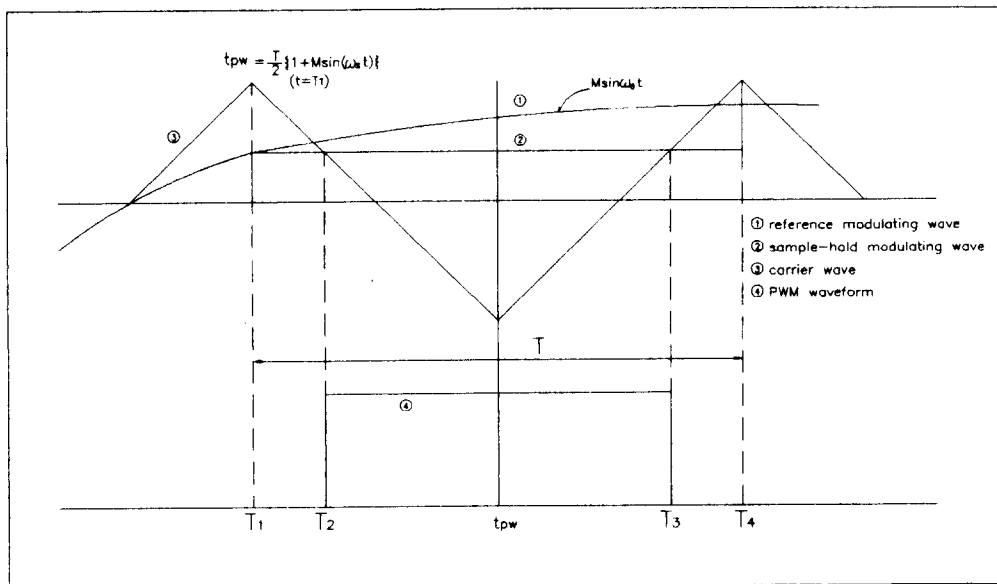
Fig. 1 Symmetric modulation waveform of RSPWM
