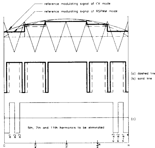
Fig. 4 PWM waveforms of RSPWM mode(a), CV mode(b) and HE mode(c)
