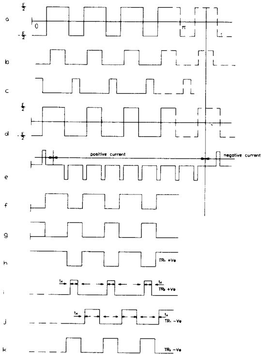
Fig. 6 Effect of TD on the inverter waveforms
