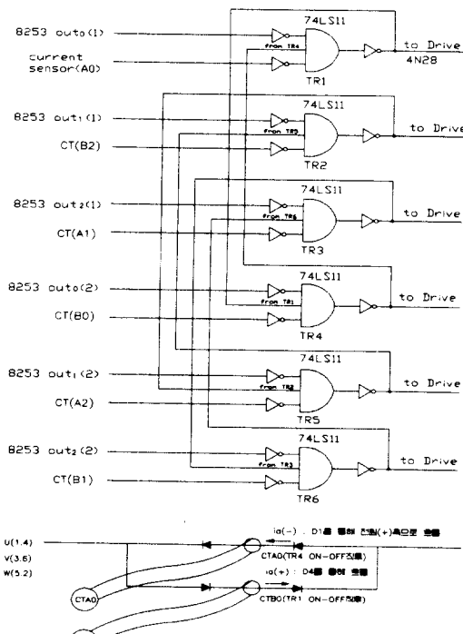
Fig. 7 TD Compensation circuit
