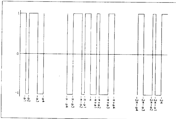
Fig. 2 Generalized output waveform of HE inverter
