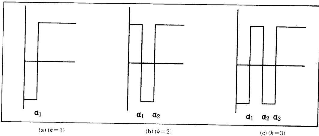
Fig.3 Firing angles and waveforms for eliminating harmonics
