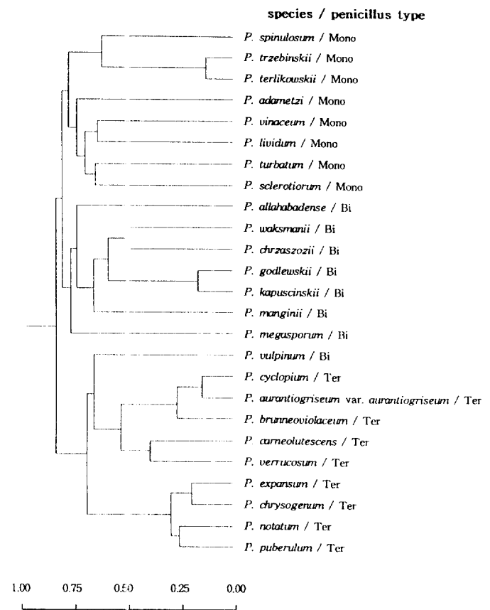
Fig. 2. Phenogram based on RAPD markers amplified from DNA of 25 Penicillium strains and 14 arbitrarily chosen 10-mer primers. The phenogram was constructed from distance values using the UPGMA method in the software package NTSYS-pc. Three distinct groups were delimited, corresponding with mono-, bi- and terverticillate species.
