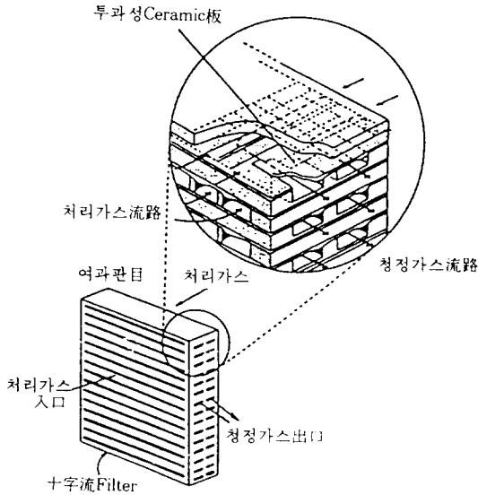
Fig. 3. Ceramic제 십자류 Filter.
