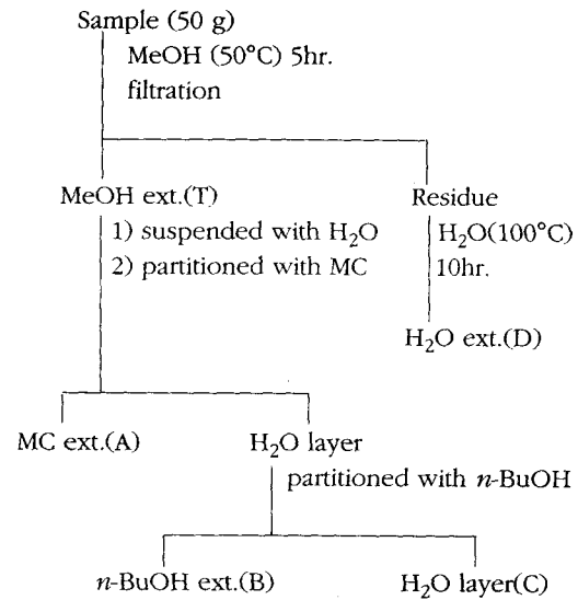
Fig. 1. Solvent fractionation of plants
