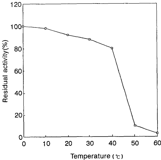
Fig. 5. Effects of temperature on stability of lipase of the molded sardine meal "koji". Crude enzyme solutions in 0.1M Na-phosphate buffer(pH 8.0) were incubated for 1hr at various temperatures.
