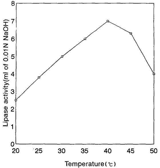
Fig. 3. Effects of temperature on lipase activity of the molded sardine meal "koji" allowed to react 60 min at pH 8.0.
