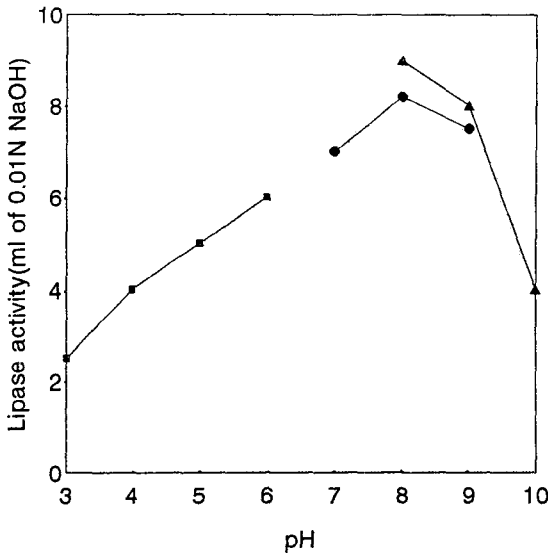
Fig. 2. Effects of pH on lipase activity of the molded sardine meal "koji" allowed to react for 60min at 37℃. (■); 0.2M acetate buffer, (●); 0.1M Tris-HCl buffer, (▲); 0.1M NH 4 OH-NH 4 Cl buffer.
