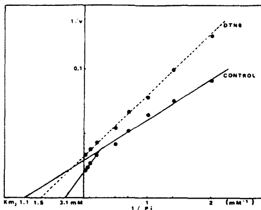
Fig. 6. Lineweaver-Burk plot of PNP treated or nontreated with DTNB with phosphate as a variable substrate.
