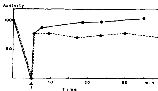
Fig. 4. Reactivation of PCMB treated PNP by thiol reagents, DTT (—) or 2-mercaptoethanol (----). The reaction mixture was prepared the same as Fig. 3. The enzyme was inactivated with 10^{-4} M PCMB for 10 min and afterwards treated with 10 mM DTT (—) or 2-mercaptoethanol (----) for the indicated incubation periods. The arrow shows the addition of thiol reagents.
