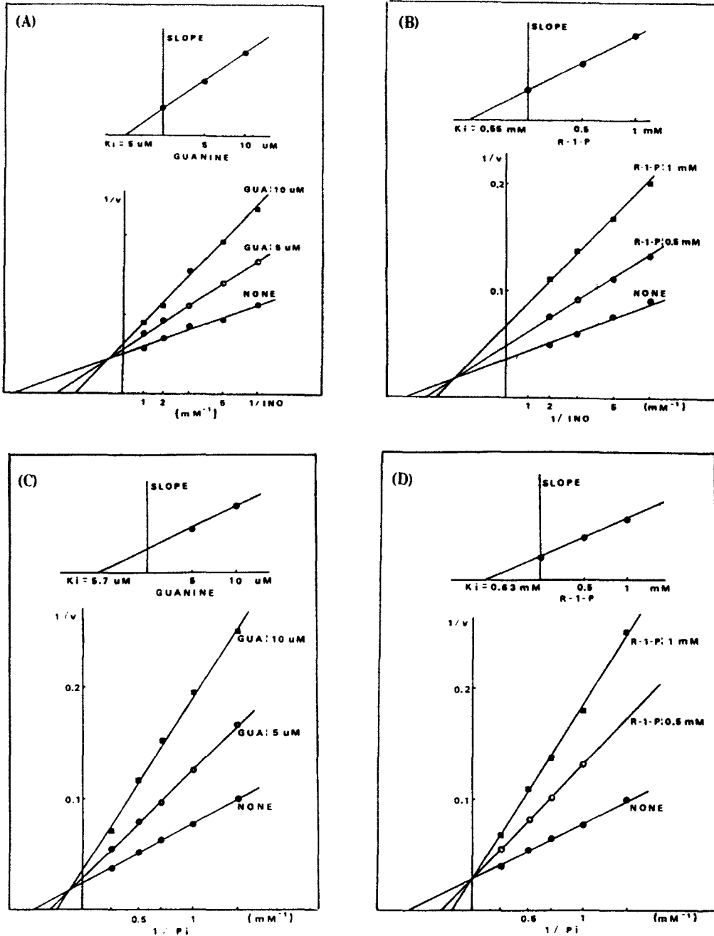
Fig. 2. Inhibition study with alternative products, guanine (A, C) or ribose 1-phosphate (B, D). Plot of reciprocal of initial velocity with respect to reciprocal of inosine (A, B) or phosphate (C, D) concentrations. The reaction mixture contained, in a final volume of 1 ml, 50 mM Tris-Cl, pH 7.3, 0.02 units of xanthine oxidase, 100 mM phosphate, the indicated amounts of inosine and alternative product, guanine (A). The reaction mixture was the same as above except 1.5 mM phosphate for alternative product, ribose 1-phosphate (B). When the phosphate concentration was varied, the reaction mixture was the same as above except 1 mM of inosine and indicated amounts of guanine (C) or ribose 1-phosphate (D).
