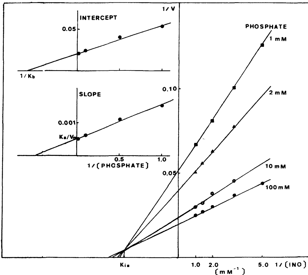
Fig. 1. The initial velocity study with inosine as the variable substrate and the plot of reciprocal velocity with respect to reciprocal of inosine concentrations.
