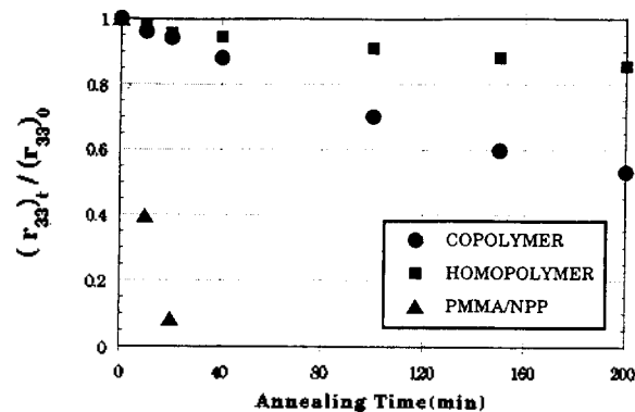
Figure 1. Relaxation behavior of r_{33} of the polymers at 80 ^{\circ}\text{C} .
