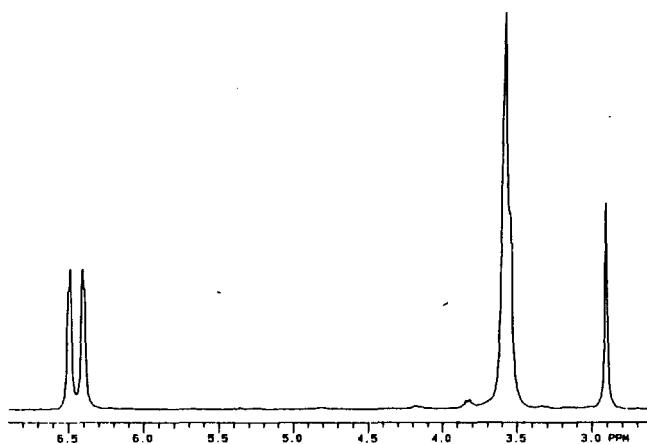
Figure 2. ^1\text{H} NMR spectrum of (\eta^5\text{-C}_5\text{H}_5)\text{Re}(\text{CO})_2\text{Br}_2^- ( 3 ) at -78^\circ\text{C} in d_8 -THF. The resonance at 3.58 ppm belongs to the THF solvent from the \text{LiEt}_3\text{BH} reducing agent.
