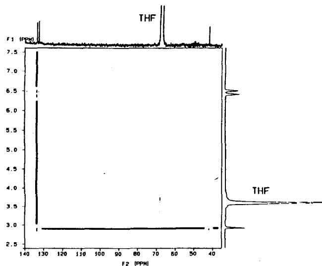
Figure 4. Long-range heteronuclear chemical shift correlation spectrum of (\eta^4\text{-C}_5\text{H}_6)\text{Re}(\text{CO})_2\text{Br}_2^- ( 3 ) at -78\text{ }^\circ\text{C} in d_8\text{-THF} .
