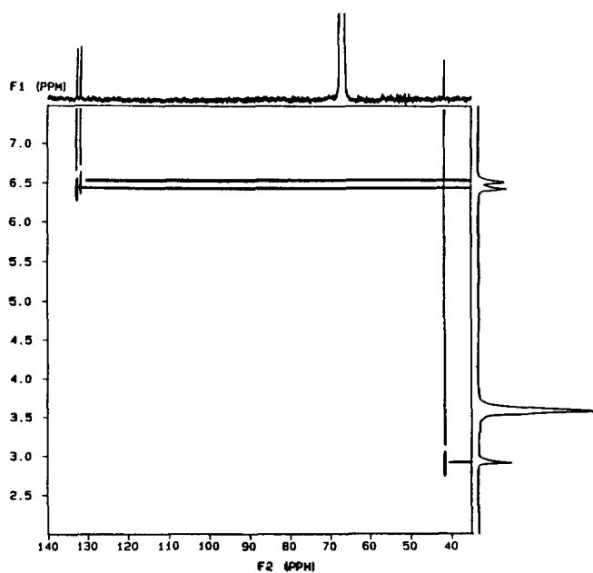
Figure 3. Heteronuclear chemical shift correlation spectrum of (\eta^5\text{-C}_5\text{H}_5)\text{Re}(\text{CO})_2\text{Br}_2^- ( 3 ) at -78^\circ\text{C} in d_8 -THF.
