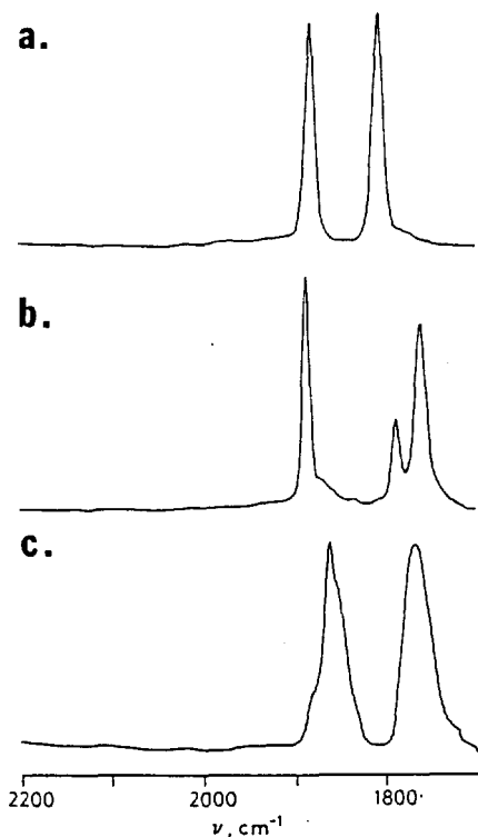
Figure 1. Infrared spectra of the carbonyl region for (a) \text{CpRe}(\text{CO})_2\text{Br}^- ( 2 ), (b) (\eta^5\text{-C}_5\text{H}_5)\text{Re}(\text{CO})_2\text{Br}_2^- ( 3 ), and (c) (\eta^5\text{-C}_5\text{H}_5)\text{Re}(\text{CO})_2\text{Br}_2^- ( 3 ) with 5 eq. of 15-Crown-5. All spectra were recorded in THF at -78^\circ\text{C} .
