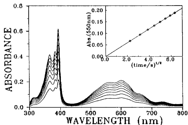
Figure 1. Absorption spectra of reduced MV^{2+} taken at potential of -0.8 V vs Ag/AgCl using an ITO glass electrode: electrolysis time, 0–40 s (step: 5s, t=0 is base line); solution, 1.0 mM MVC_2 and 0.1 M KCl in H_2O . Inset shows absorbances at 550 nm vs (electrolysis time/s) ^{1/2} .
