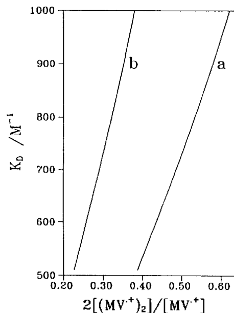
Figure 3. Calculated working curves for K_D vs 2[(MV^+)_2]/[MV^+] for bulk [MV^{2+}] = 1.0 (a) and 0.5 mM (b). Note that 2[\text{dimer}]/[\text{monomer}] corresponds to the absorbance ratio ( A_{\text{dimer}}/A_{\text{monomer}} ) of the resolved spectra at the isosbestic point, 550 nm.
