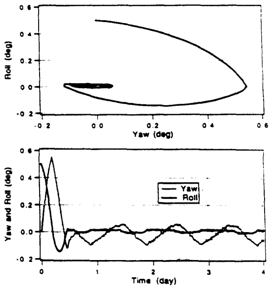
Figure 7. Roll angle acquisition performance
