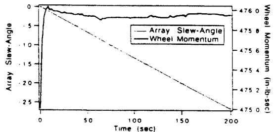
Figure 13. Pitch response during array slew (1 in-lb-sec = 1.152 cm-kg-sec)
