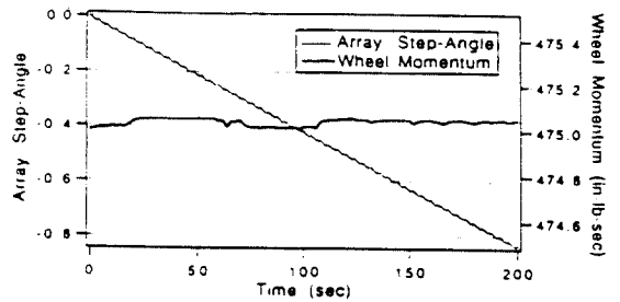
Figure 12. Nominal pitch loop performance (1 in-lb-sec = 1.152 cm-kg-sec)
