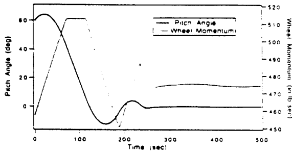
Figure 11. Pitch capture at momentum offset (1 in-lb-sec = 1.152 cm-kg-sec)
