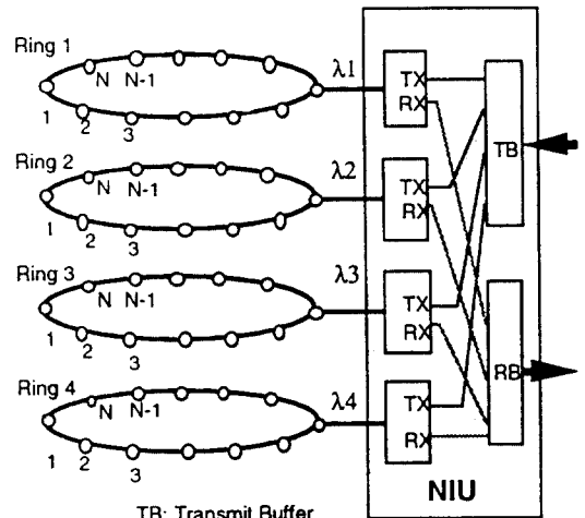
(a) A Topological View of a Shared Configuration of a 4 WDM Channel Ring.
