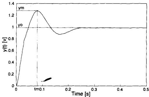
Fig. 2-5. Step response of the cart control system.
