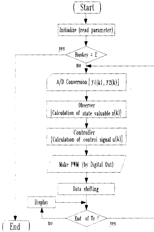
Fig. 4-2. Flow chart of control algorithm.
