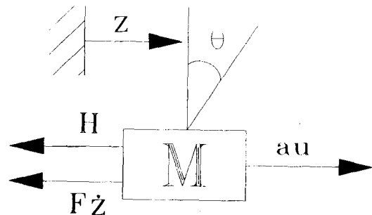
Fig. 2-1. The motion of cart.
