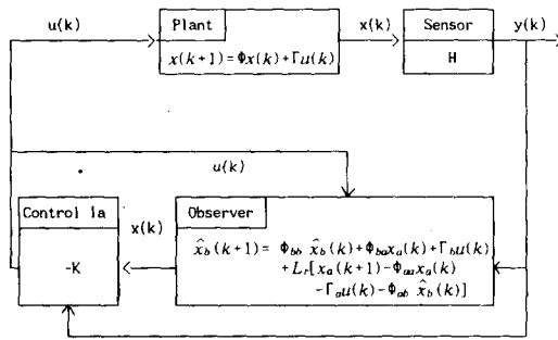
Fig. 3-1. Block diagram of LQR control system.
