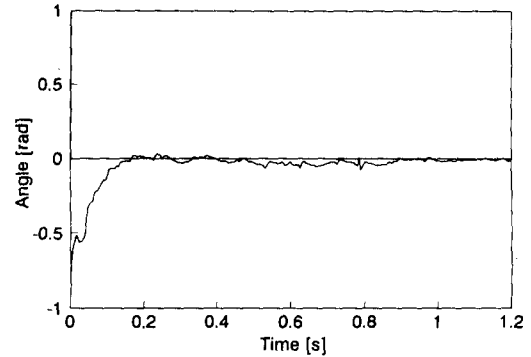
Fig. 5.1. Step response.
