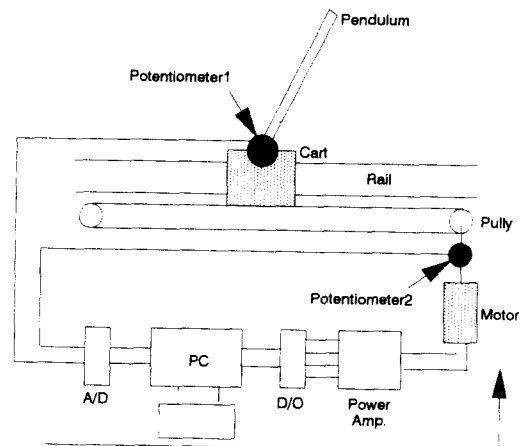
Fig. 2-3. Schematic diagram of experimental apparatus.
