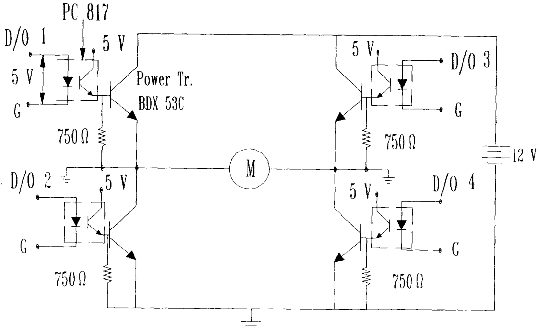
Fig. 4-1. Driving circuit of DC servo motor.
