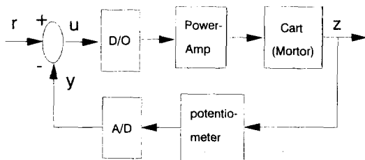
Fig. 2-4. Block diagram of cart control system for identification of parameter.
