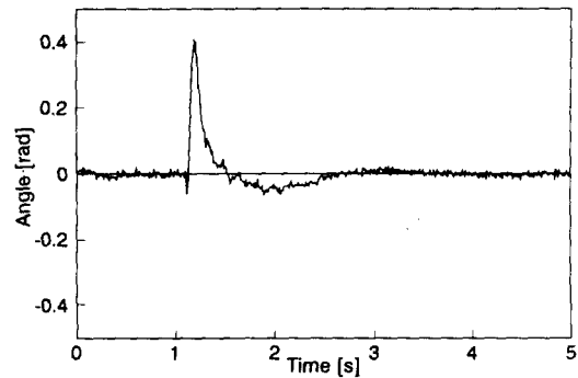
Fig. 5.2. Response under disturbance.
