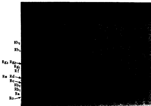
Fig. 1. Thin layer chromatograms of saponin components from nonirradiated and irradiated red ginseng. Sample were as follows: 1~3, 0 time 14% control, 5 kGy and 10 kGy; 4~6, 0 time 18% control, 5 kGy and 10 kGy; 7~9, 20°C 6 month 14% control, 5 kGy and 10 kGy; 10~12, 20°C 6 month 18% control, 5 kGy and 10 kGy; 13~15, 40°C 6 month 14% control, 5 kGy and 10 kGy; 16~18, 40°C 6 month 18% control, 5 kGy and 10 kGy, respectively.
