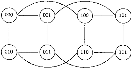
a) 3-dimensional hypercube
