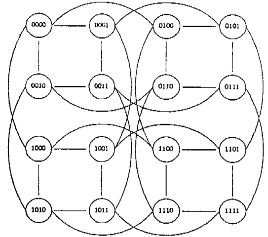
a) 4-dimensional hypercube
