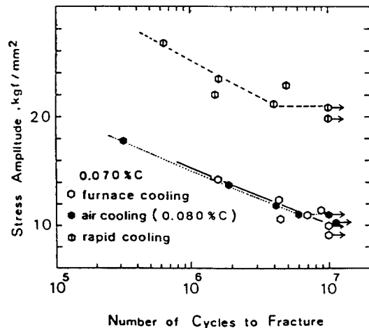
Fig. 7 Fatigue test results of 0.070 and 0.080% C specimens
