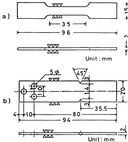
Fig. 1 Shape and dimension of test specimens a) tension test specimen b) fatigue test specimen
