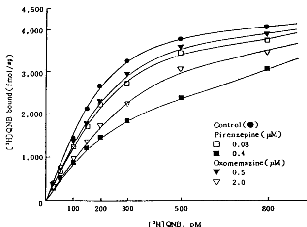
Fig. 4. Effect of pirenzepine and oxomemazine on the saturation isotherms of [ 3 H]QNB binding to rat cerebral microsome. Cerebral microsomes (0.05 mg protein) were incubated with increasing concentration of [ 3 H]QNB in the absence of unlabeled drug (●) or presence of pirenzepine (□: 0.08 μM, ■: 0.4 μM) or oxomemazine (▼: 0.5 μM, ▽: 2 μM). Nonspecific binding was defined in the presence of 10 μM atropine. The data shown are the result obtained from three independent experiments.
