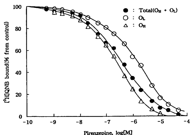
Fig. 6. Pirenzepine/ [^3\text{H}] QNB competition binding to the total population ( O_H+O_L , ●), the O_L sites (○) and the O_H sites (△). Competition binding for the O_L sites was performed in the presence of 8 \mu\text{M} oxomemazine. The competition binding data for O_H sites were calculated by subtracting the curve for O_L sites from the total curves. Each point represents the mean of three independent experiments.
