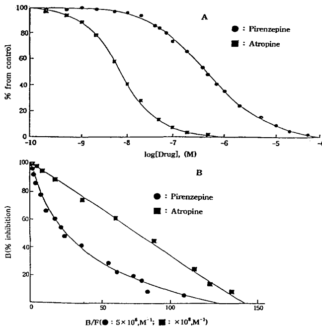
Fig. 2. Inhibition of [ ^3\text{H} ]QNB binding by atropine and pirenzepine to rat cerebral microsome. The concentration of [ ^3\text{H} ]QNB was 300 pM. A: Inhibition curve of atropine (■) and pirenzepine (●) with [ ^3\text{H} ]QNB. B: Hofstee plot of the inhibition data. B represents the percentage inhibition of [ ^3\text{H} ]QNB binding and F the free pirenzepine or atropine concentration. Each point represents the mean of four separate determinations.
