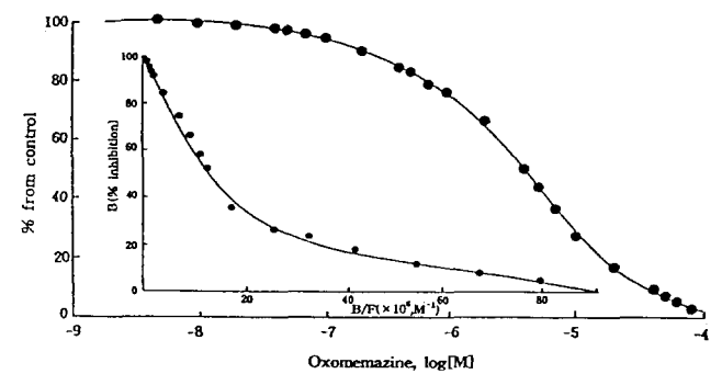
Fig. 3. Inhibition of [ ^3\text{H} ]QNB binding by oxomemazine to rat cerebral microsome. The concentration of [ ^3\text{H} ]QNB was 300 pM. Inset: Hofstee plot of the competition binding data. Each point represents the mean of eight separate determinations.
