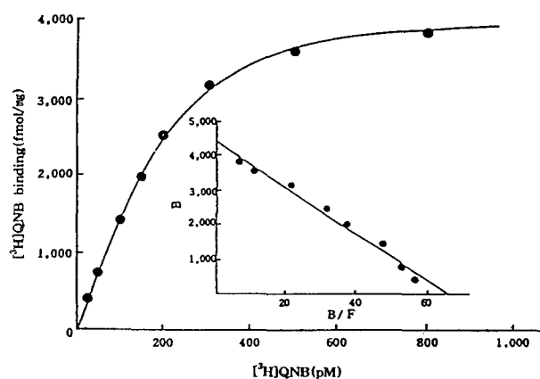
Fig. 1. A typical saturation experiment with [ 3 H]QNB in rat cerebral microsome. Microsomal protein (50 μg) was incubated with various concentrations of [ 3 H]QNB for 150 min at 37°C in a final volume of 1 ml. The inset shows a Scatchard plot of specific [ 3 H]QNB binding. Bound [ 3 H]QNB(B) was plotted as a function of bound [ 3 H]QNB(B)/free [ 3 H]QNB(F).
