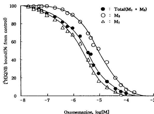
Fig. 5. Oxomemazine/[ 3 H]QNB competition binding to the total population (M 1 +M 3 , ●), M 3 (○) and M 1 (△) receptors. Competition binding for M 3 was performed in the presence of 2 μM pirenzepine. The competition binding data for M 1 were calculated by subtracting the curve for M 3 from the total curves. Each point represents the mean of four independent experiments.
