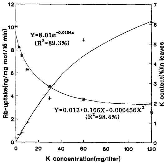
Fig. 5. Change of Rb-uptake and K content in leaves of Hordeum distichum grown at the different K concentrations of the water culture solution.
